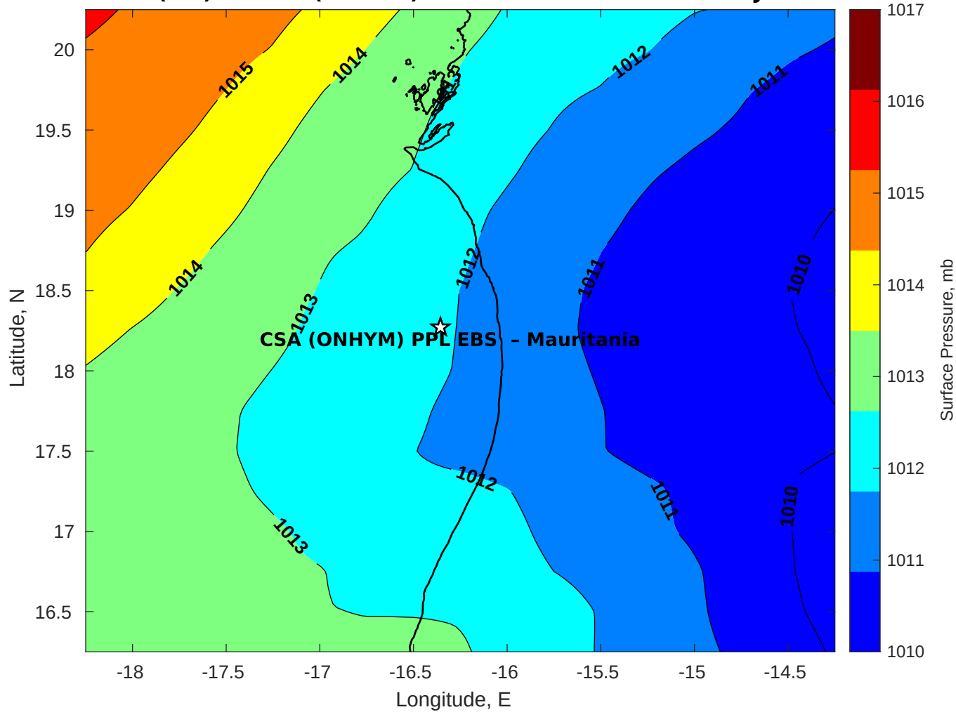
Surface Pressure (mb) for CSA (ONHYM) PPL EBS - Mauritania at 09-Jun-2025 00:00:00
