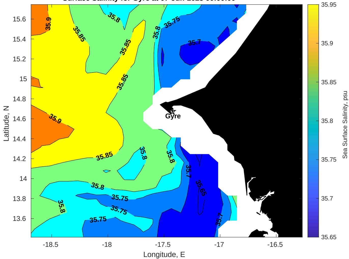
Surface Salinity for Gyre at 07-Jun-2025 00:00:00
