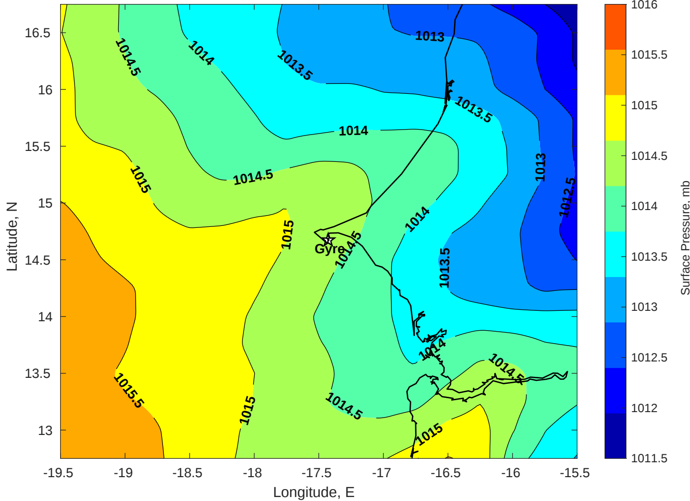
Surface Pressure (mb) for Gyre at 09-Jun-2025 00:00:00
