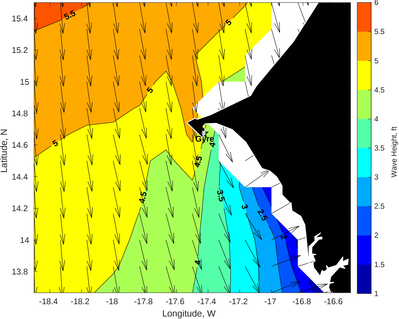
Wave Height (ft) for Gyre at 08-Jun-2025 09:00:00
