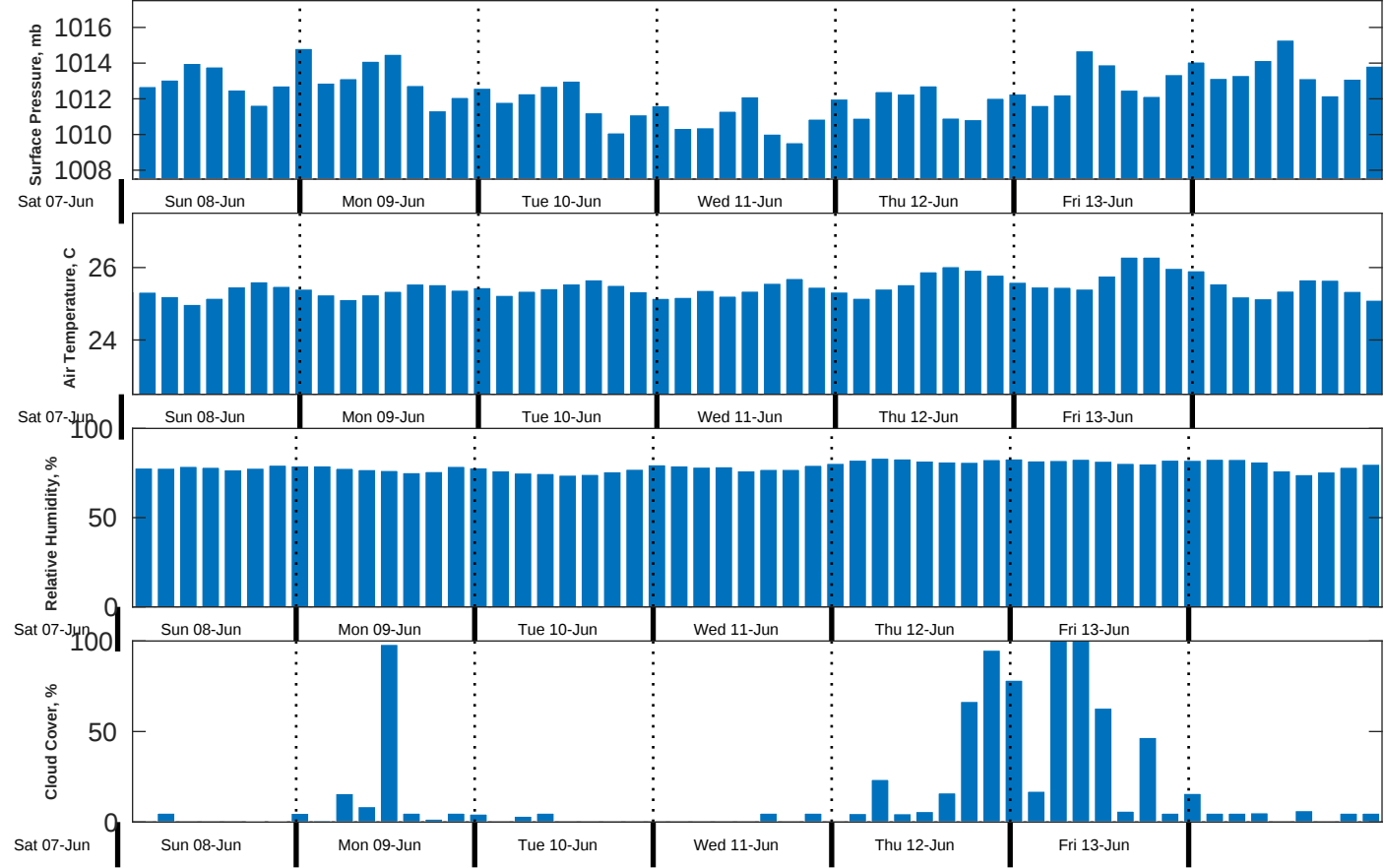
Met Forecast for Gyre from 07-Jun-2025 23:00:00 to 14-Jun-2025 23:00:00
