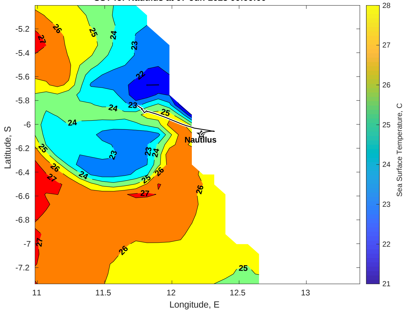
SST for Nautilus at 07-Jun-2025 00:00:00
