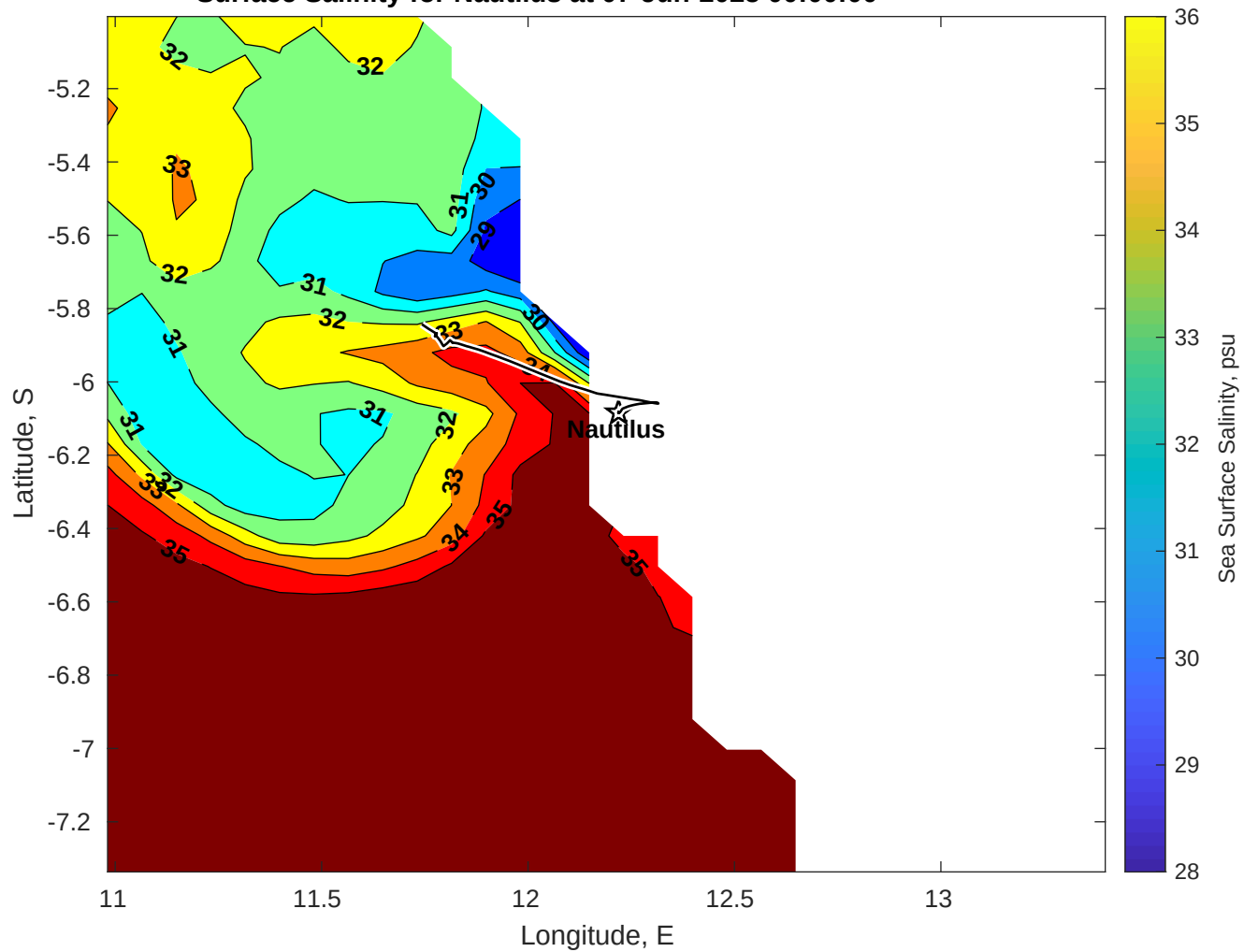
Surface Salinity for Nautilus at 07-Jun-2025 00:00:00
