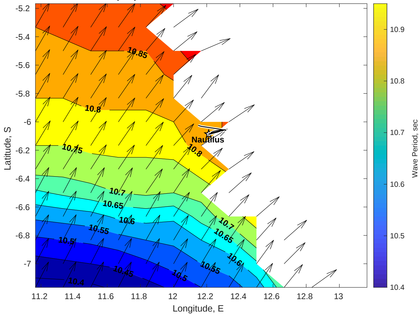
Wave Period (sec) for Nautilus at 08-Jun-2025 09:00:00
