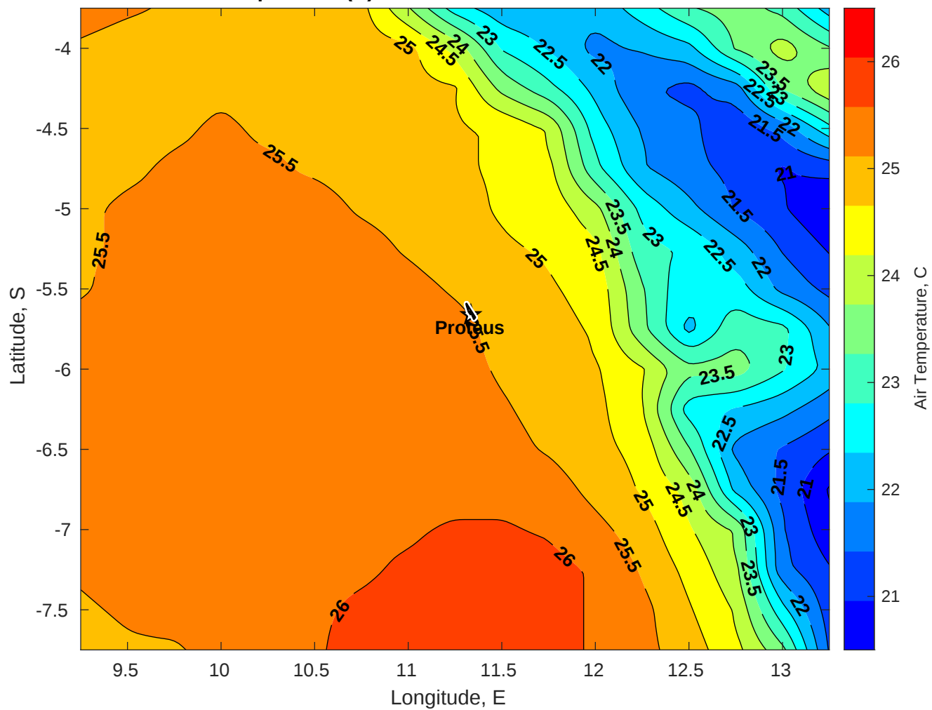
Air Temperature (C) for Proteus at 08-Jun-2025
