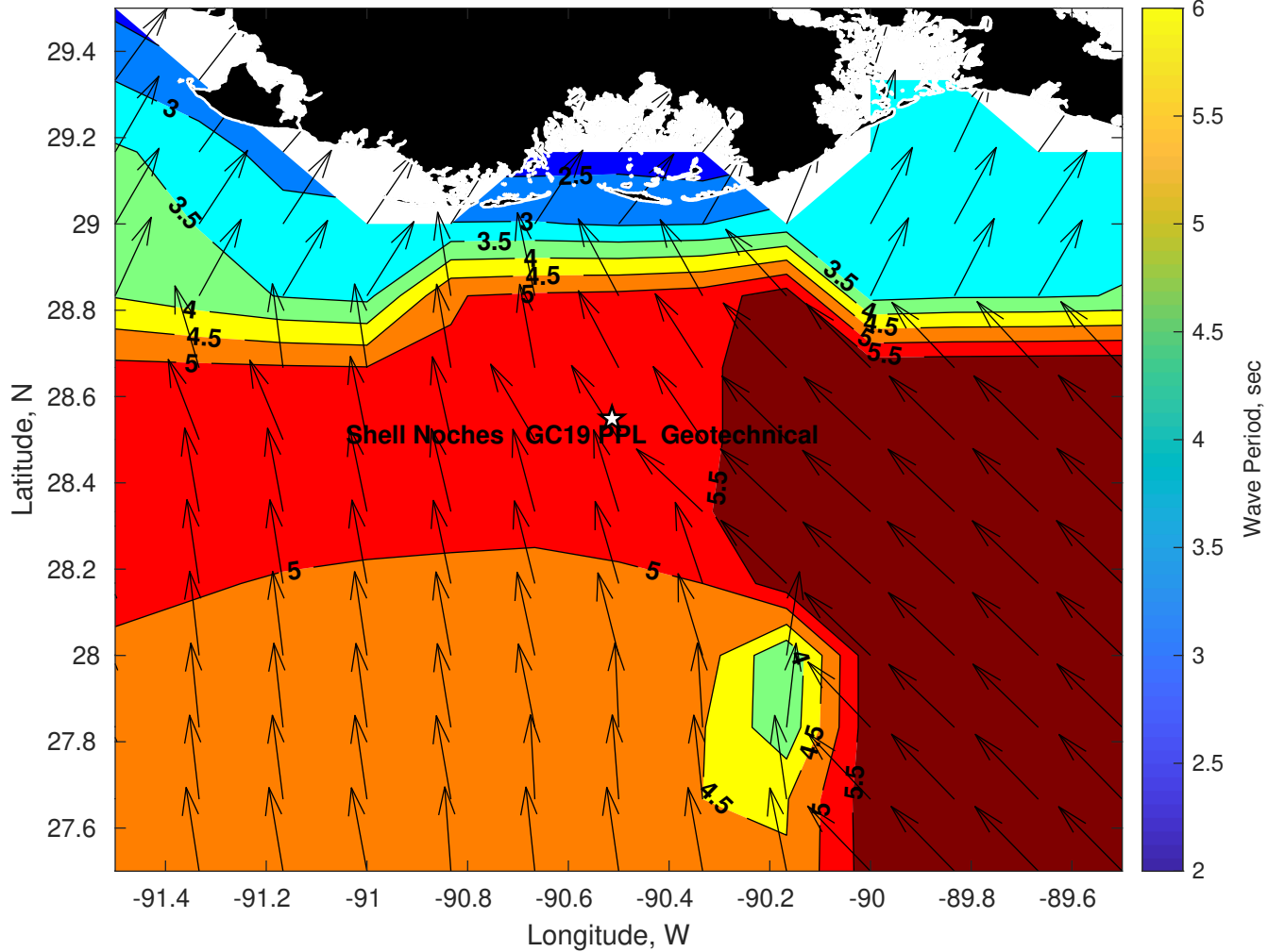
Wave Period (sec) for Shell Noches GC19 PPL Geotechnical at 08-Jun-2025 09:00:00
