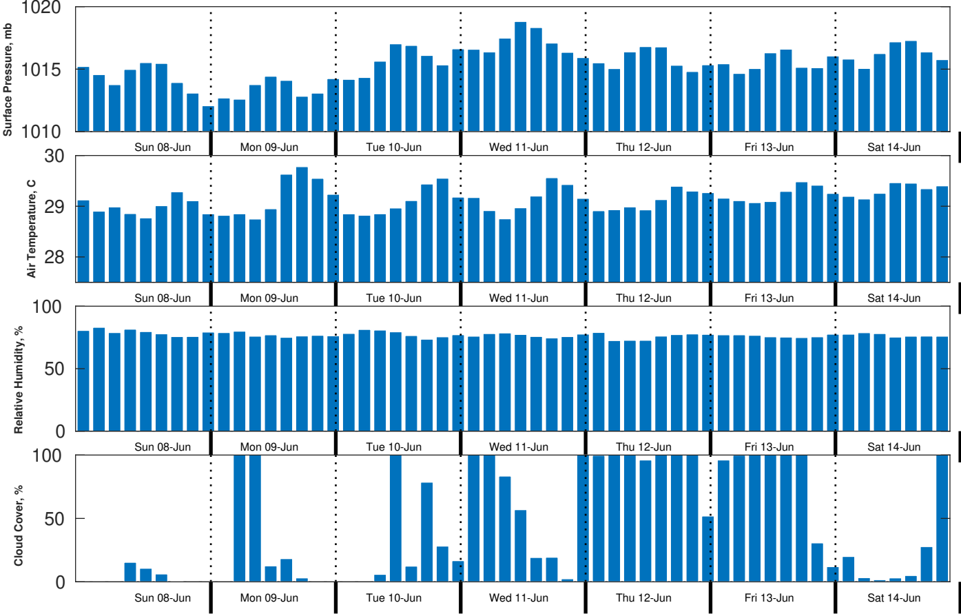
Met Forecast for Shell Noches GC19 PPL Geotechnical from 08-Jun-2025 00:00:00 to 15-Jun-2025 00:00:00
