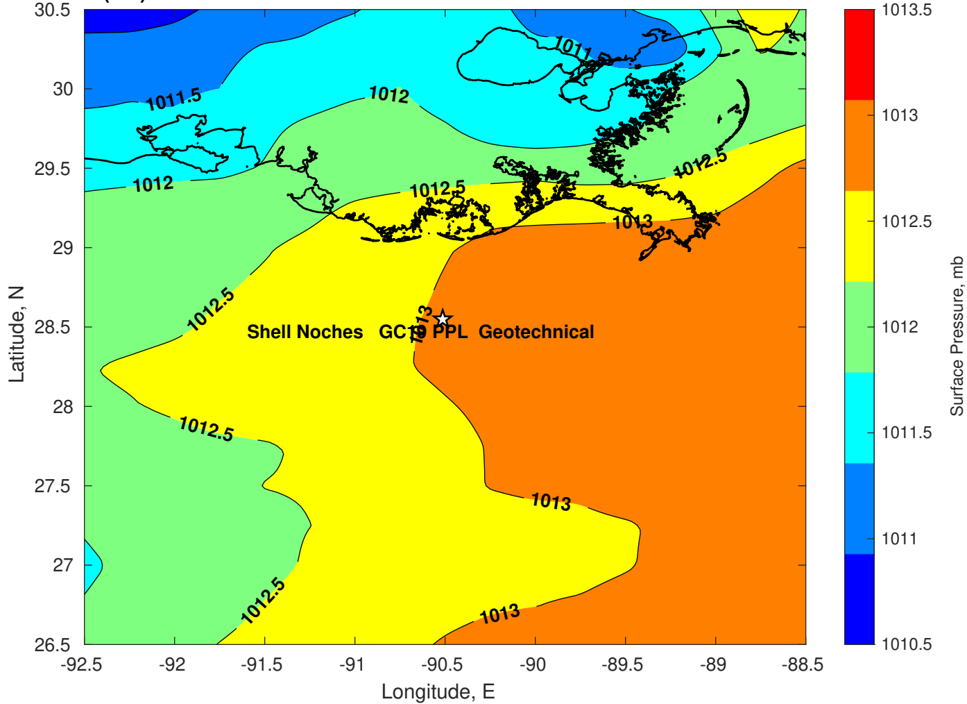
Surface Pressure (mb) for Shell Noches GC19 PPL Geotechnical at 10-Jun-2025 00:00:00
