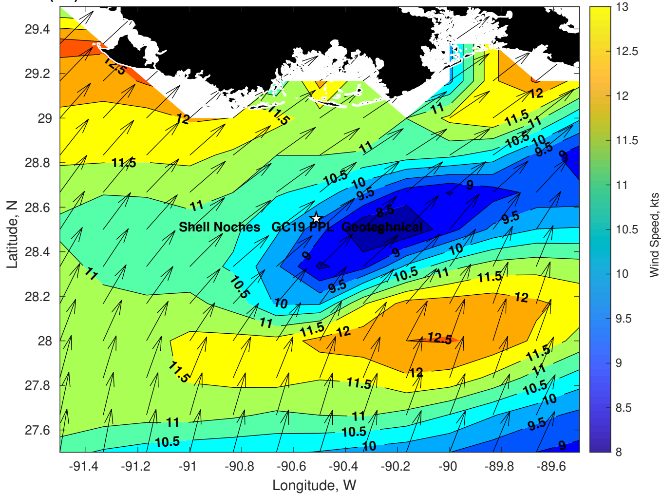
Winds (kts) for Shell Noches GC19 PPL Geotechnical at 08-Jun-2025 09:00:00
