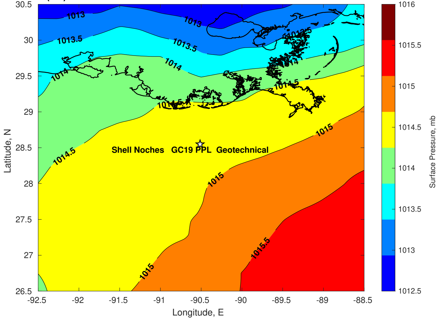
Surface Pressure (mb) for Shell Noches GC19 PPL Geotechnical at 08-Jun-2025 00:00:00
