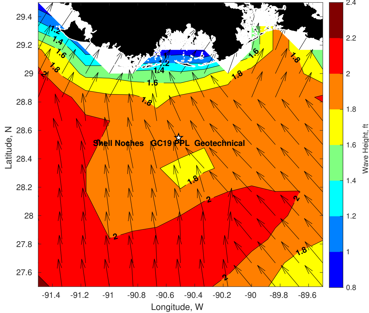
Wave Height (ft) for Shell Noches GC19 PPL Geotechnical at 08-Jun-2025 09:00:00
