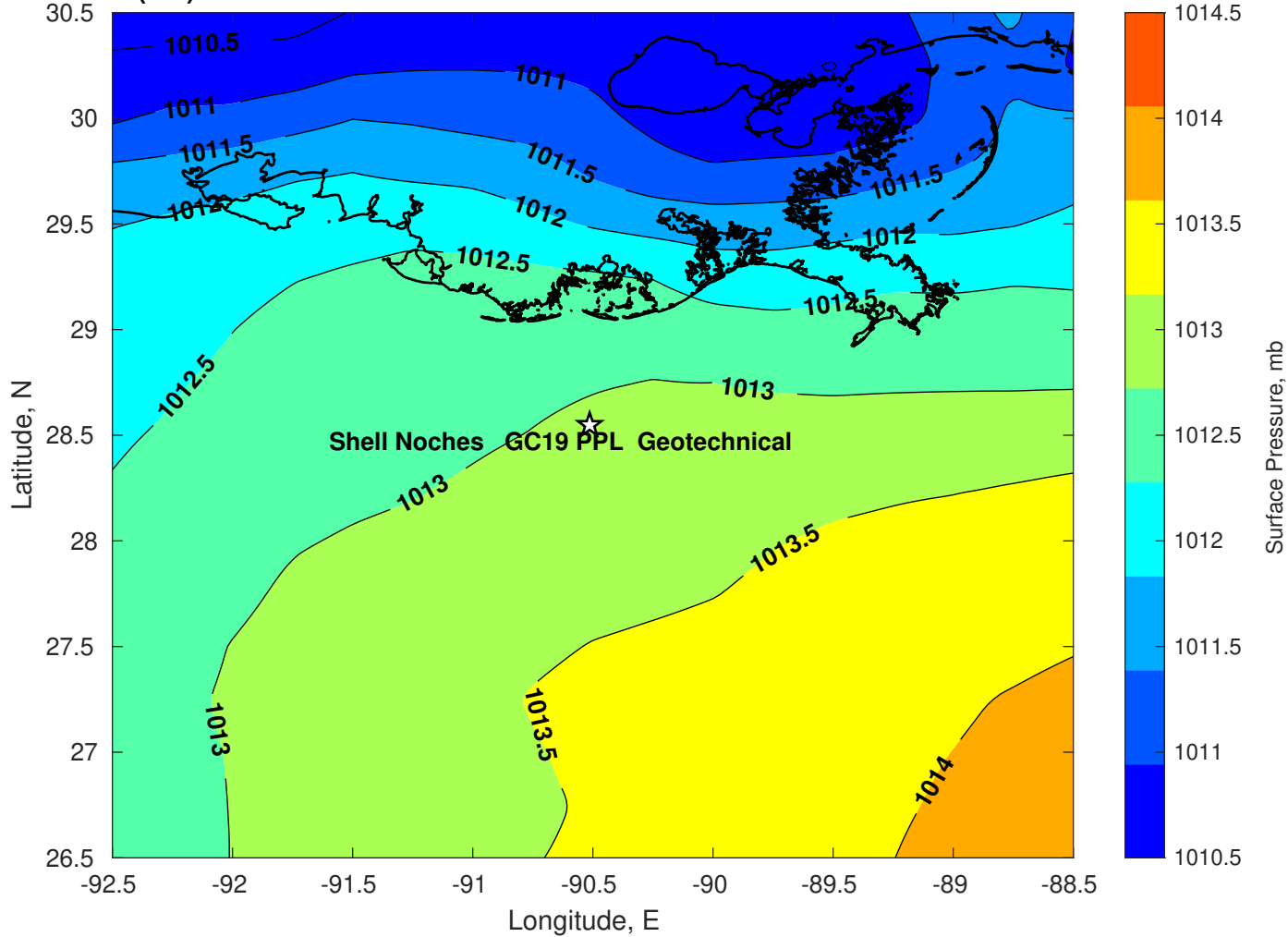
Surface Pressure (mb) for Shell Noches GC19 PPL Geotechnical at 09-Jun-2025 00:00:00
