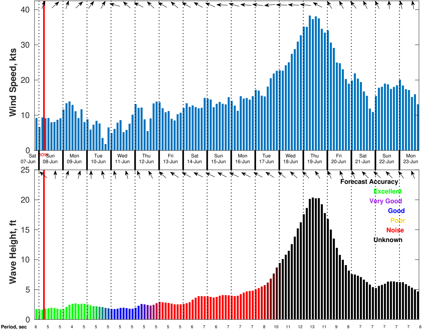
Wind & Wave Forecast for Shell Noches GC19 PPL Geotechnical from 07-Jun-2025 20:00:00 to 23-Jun-2025 20:00:00
