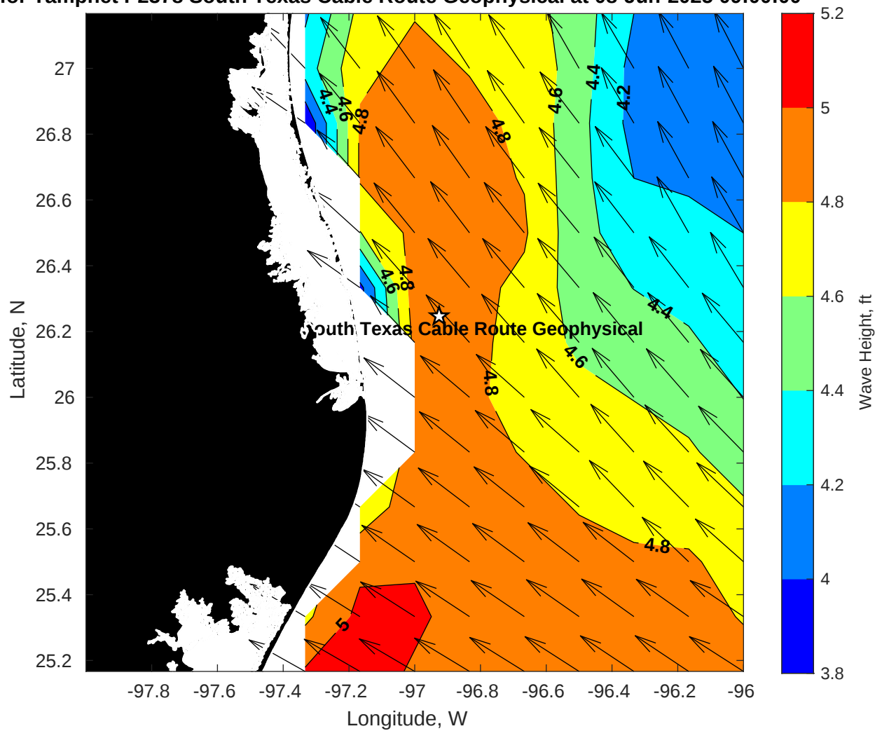
Wave Height (ft) for Tampnet P2378 South Texas Cable Route Geophysical at 08-Jun-2025 09:00:00
