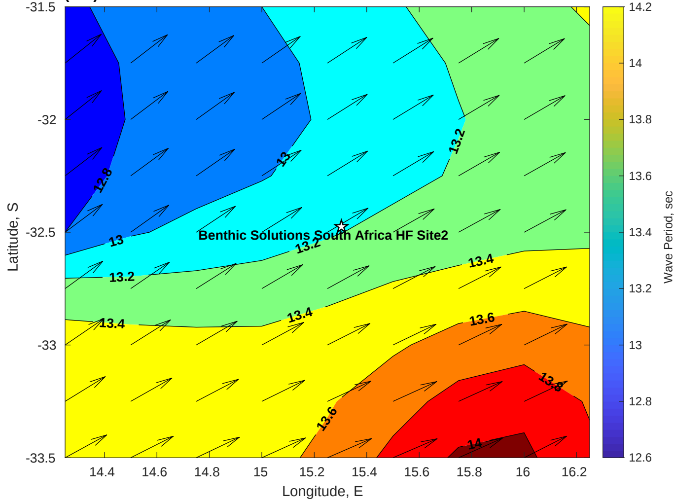
Wave Period (sec) for Benthic Solutions South Africa HF Site2 at 08-Jun-2025 09:00:00
