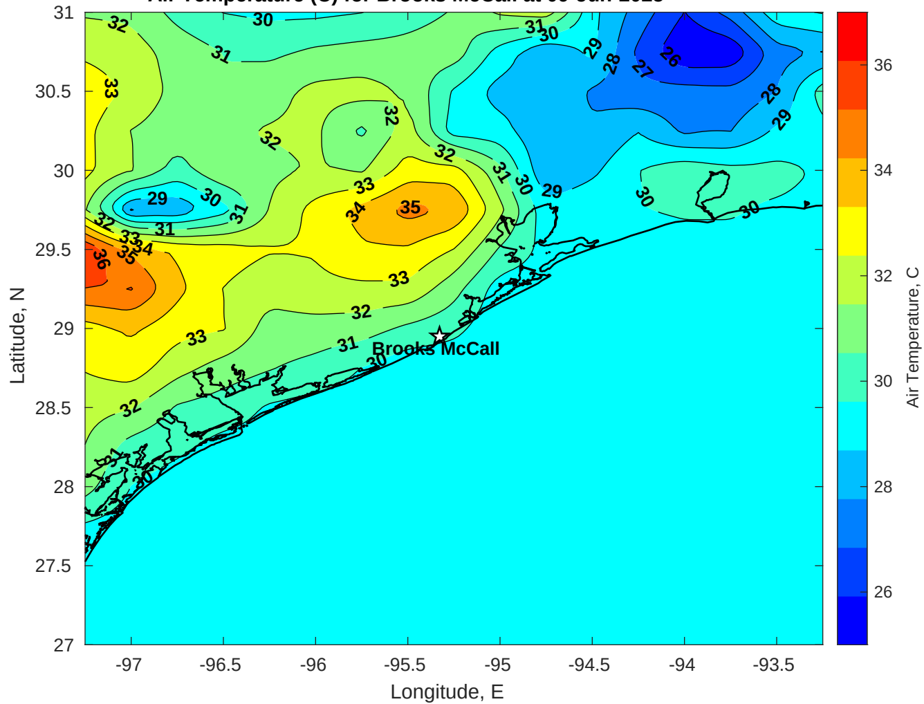
Air Temperature (C) for Brooks McCall at 09-Jun-2025
