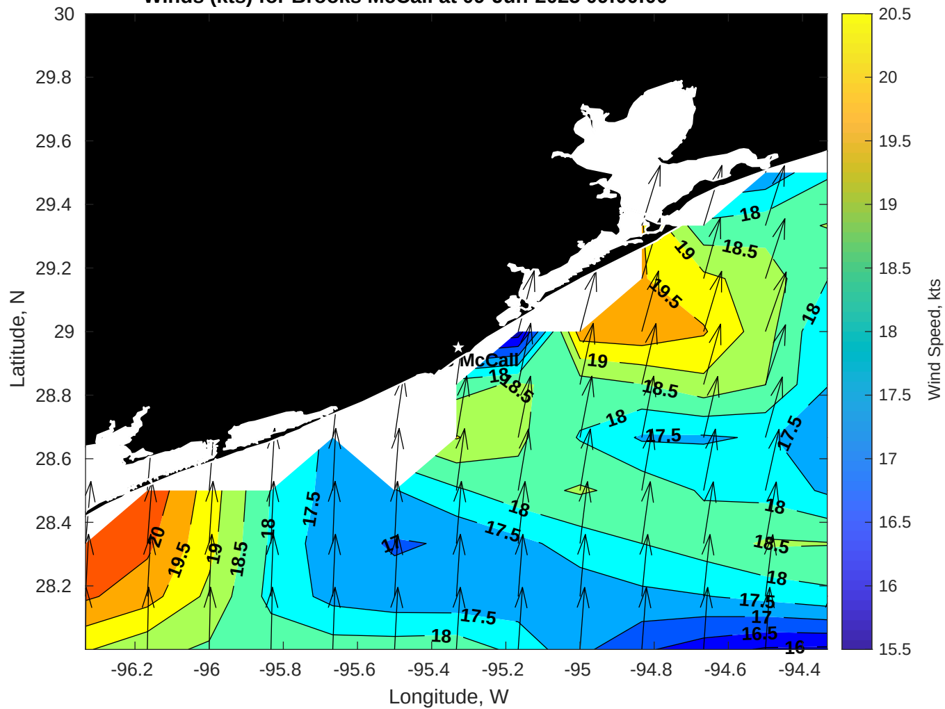
Winds (kts) for Brooks McCall at 09-Jun-2025 09:00:00
