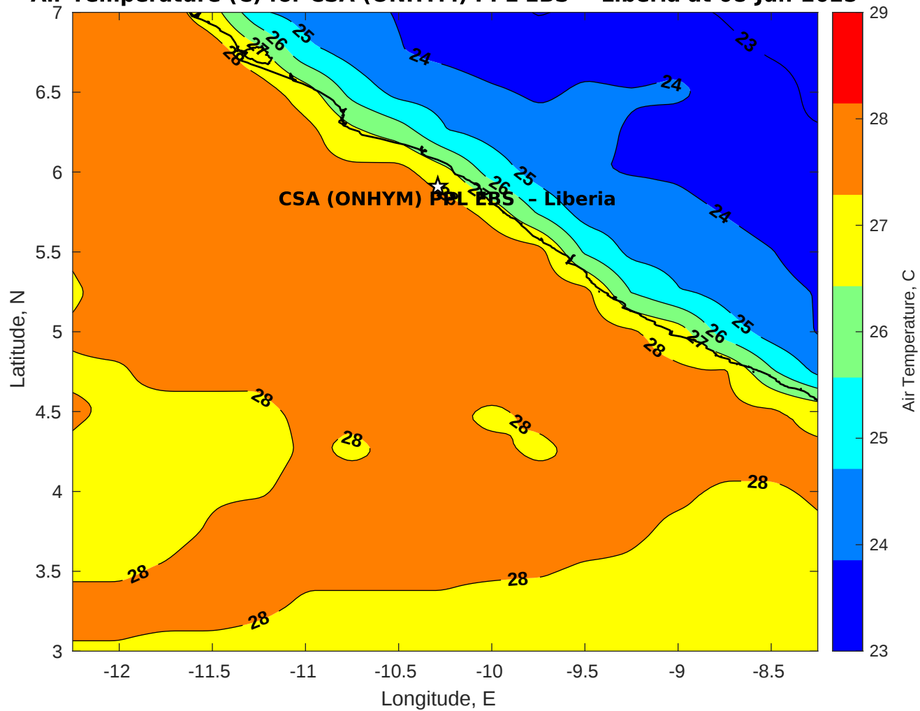
Air Temperature (C) for CSA (ONHYM) PPL EBS - Liberia at 08-Jun-2025
