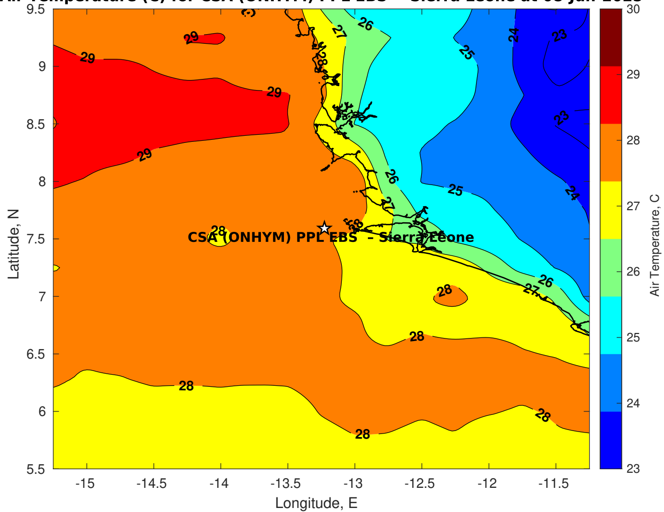
Air Temperature (C) for CSA (ONHYM) PPL EBS - Sierra Leone at 08-Jun-2025
