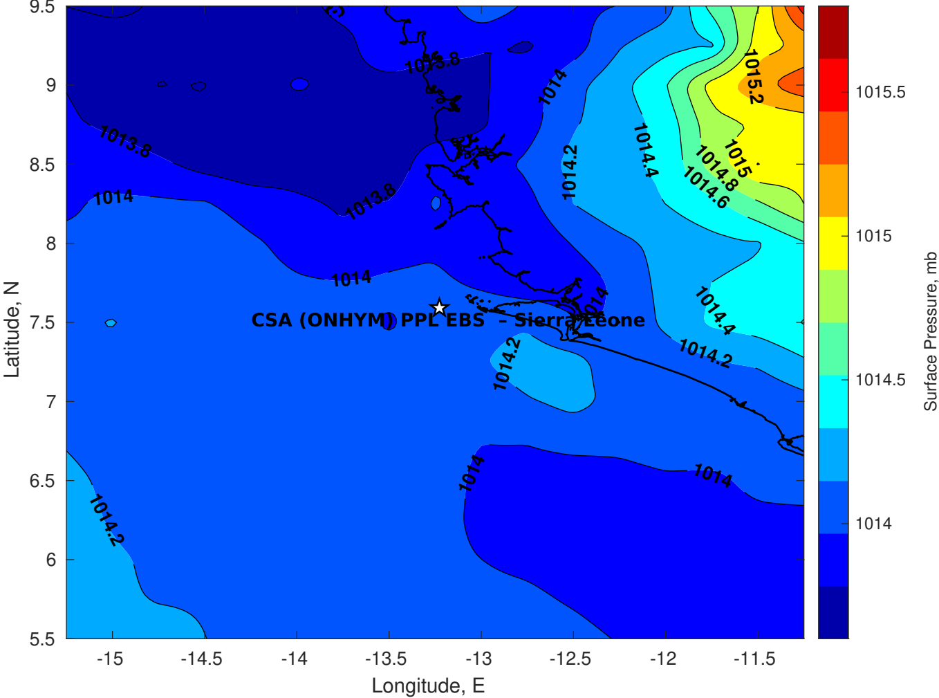
Surface Pressure (mb) for CSA (ONHYM) PPL EBS - Sierra Leone at 10-Jun-2025 00:00:00
