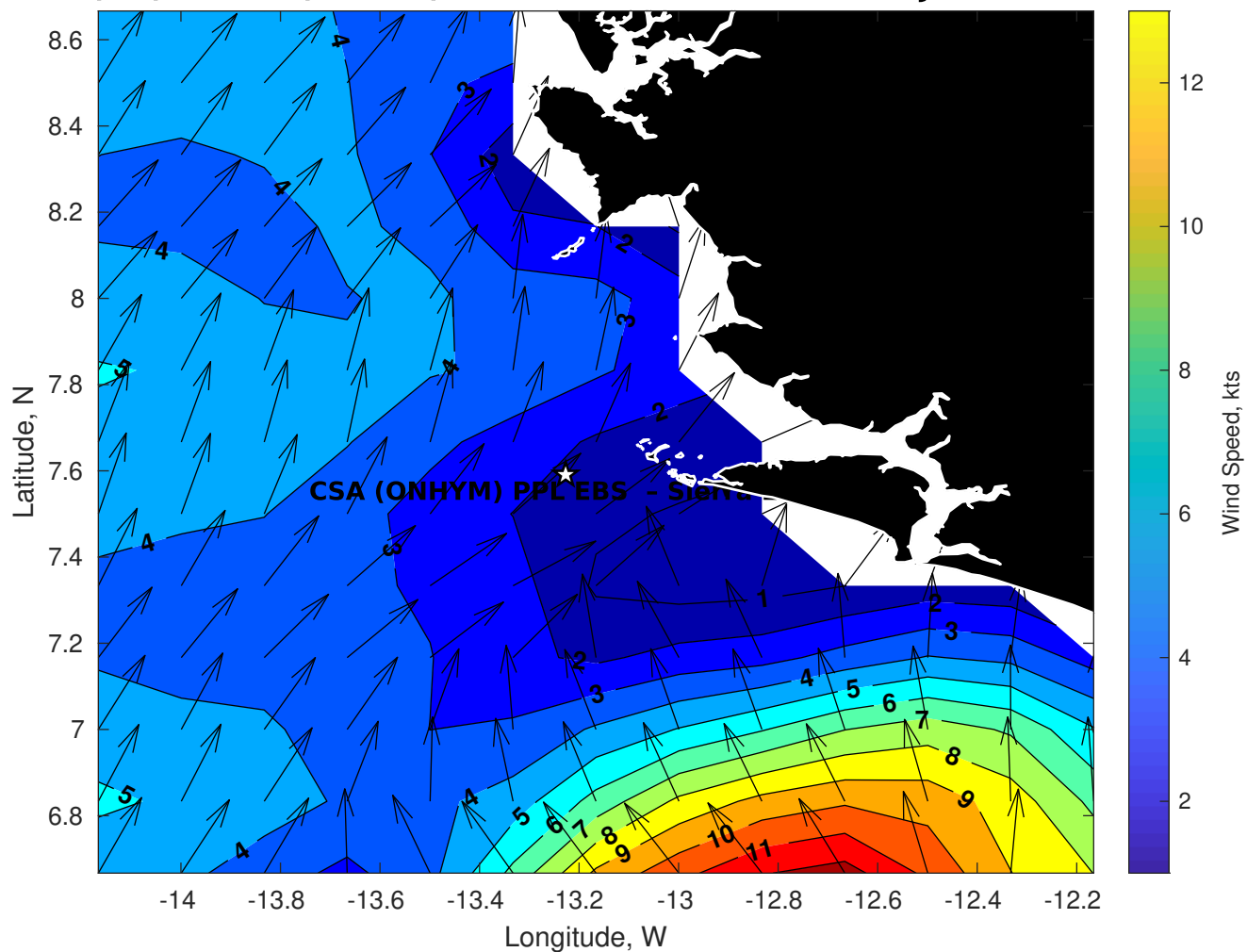
Winds (kts) for CSA (ONHYM) PPL EBS - Sierra Leone at 08-Jun-2025 09:00:00
