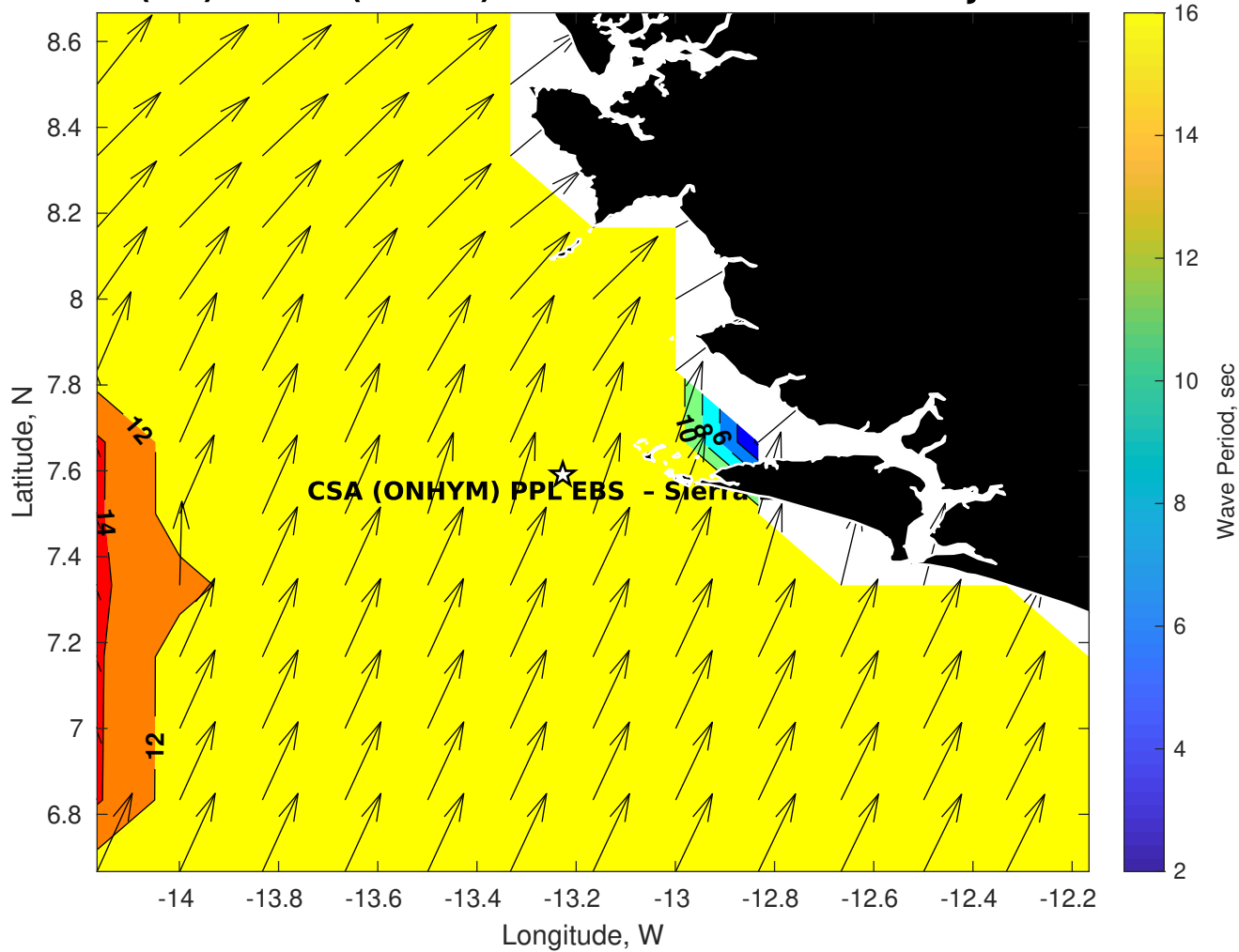
Wave Period (sec) for CSA (ONHYM) PPL EBS - Sierra Leone at 08-Jun-2025 09:00:00
