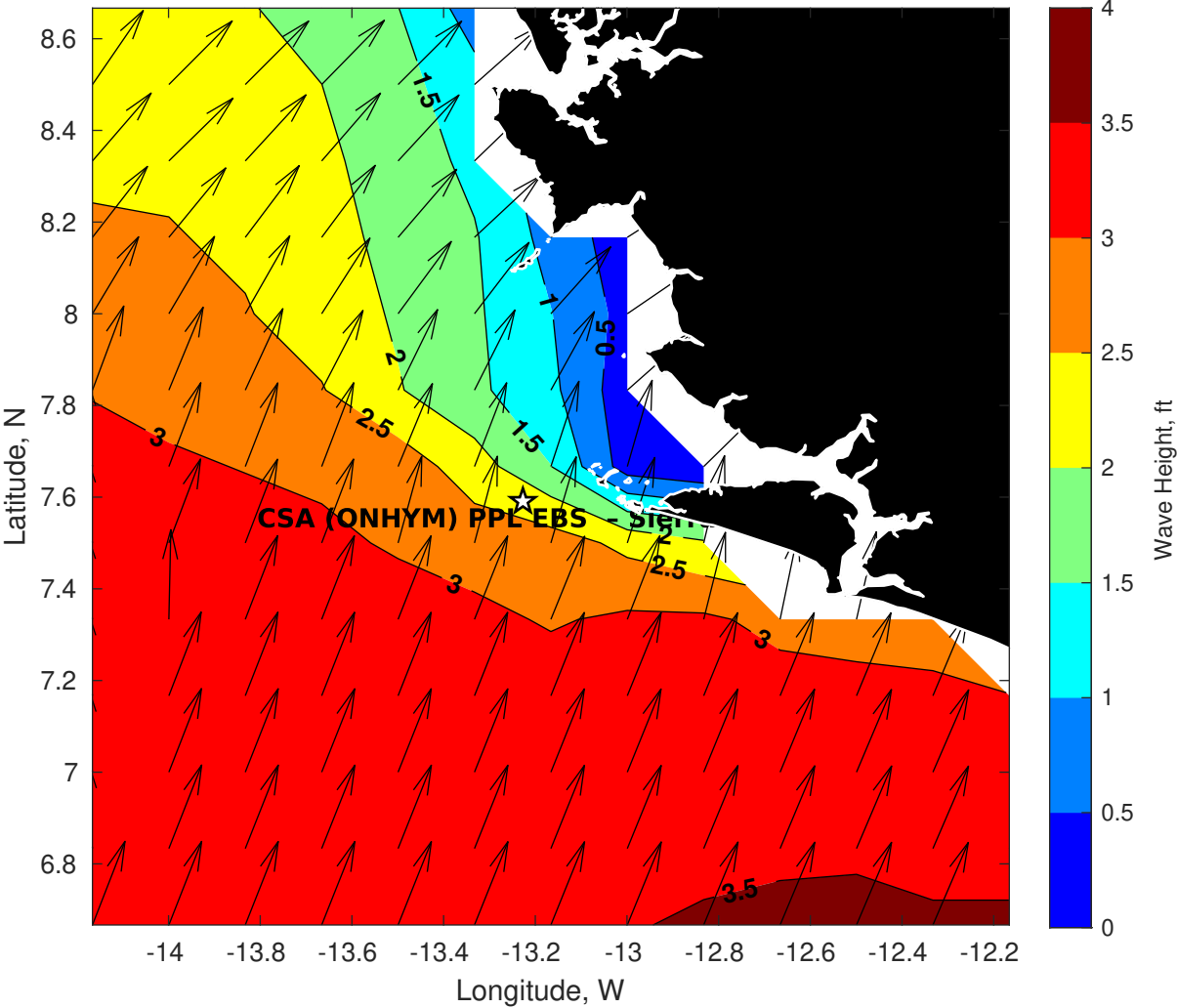
Wave Height (ft) for CSA (ONHYM) PPL EBS - Sierra Leone at 08-Jun-2025 09:00:00
