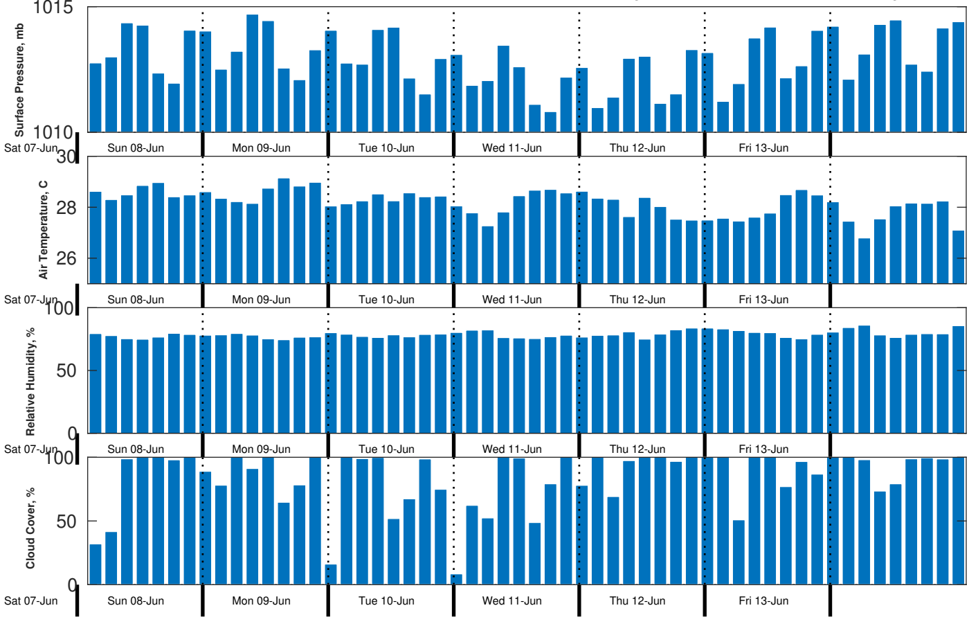
Met Forecast for CSA (ONHYM) PPL EBS - Sierra Leone from 08-Jun-2025 00:00:00 to 15-Jun-2025 00:00:00
