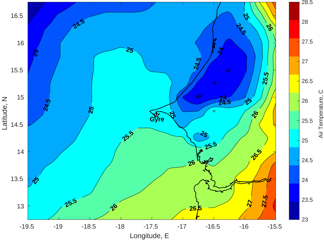
Air Temperature (C) for Gyre at 09-Jun-2025
