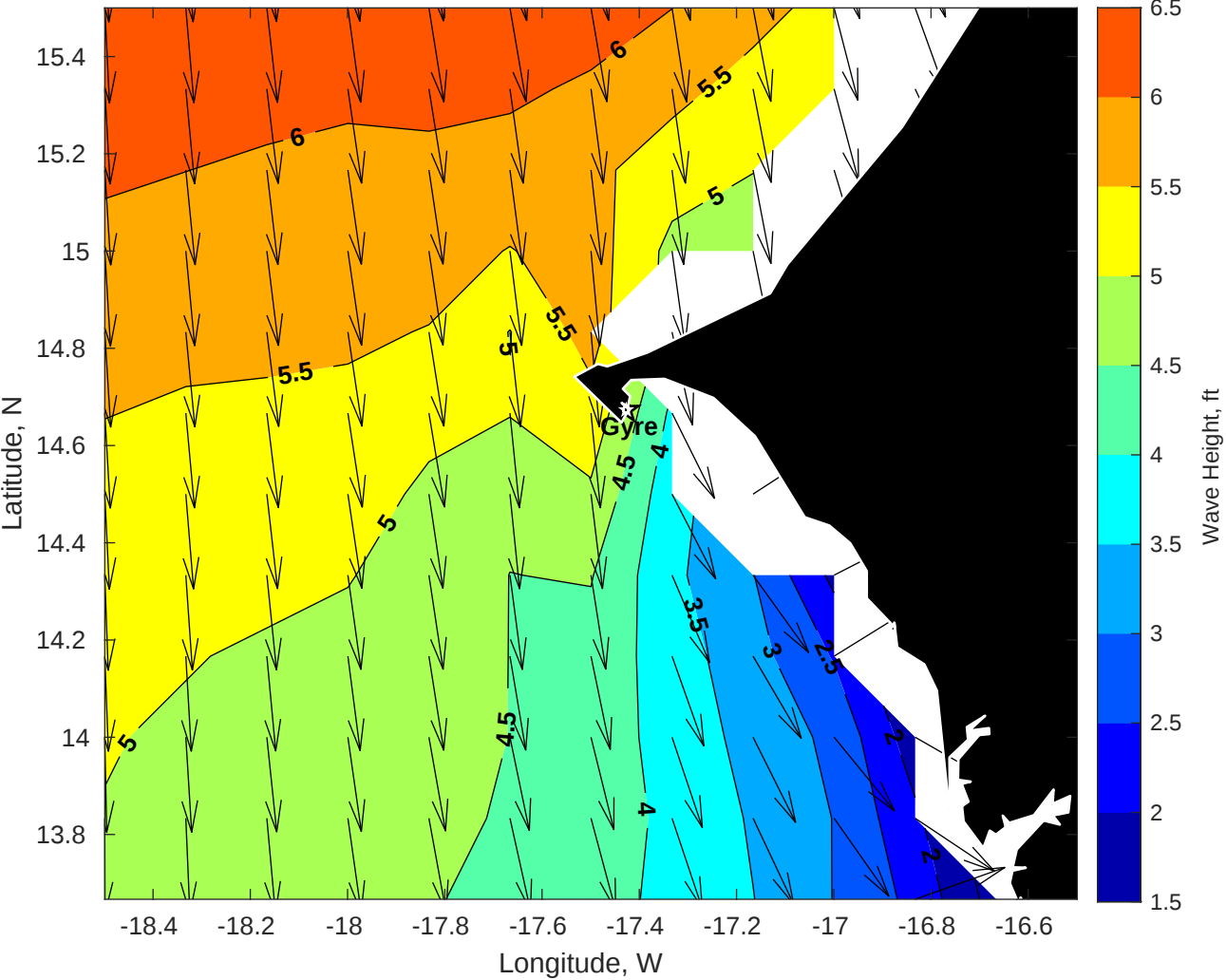
Wave Height (ft) for Gyre at 09-Jun-2025 09:00:00
