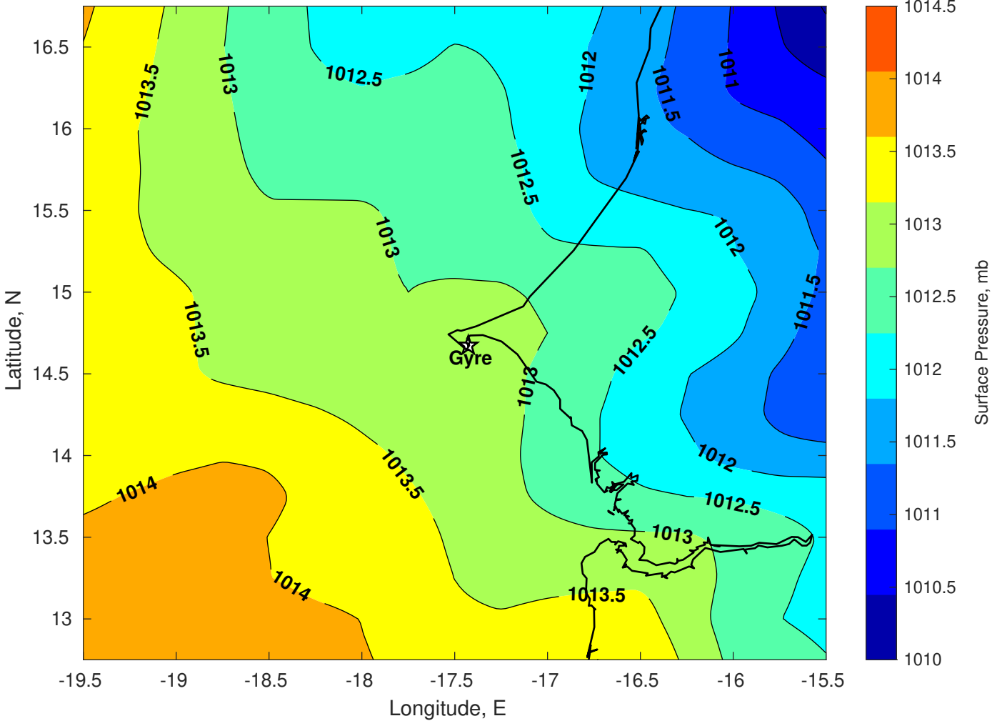
Surface Pressure (mb) for Gyre at 10-Jun-2025 00:00:00
