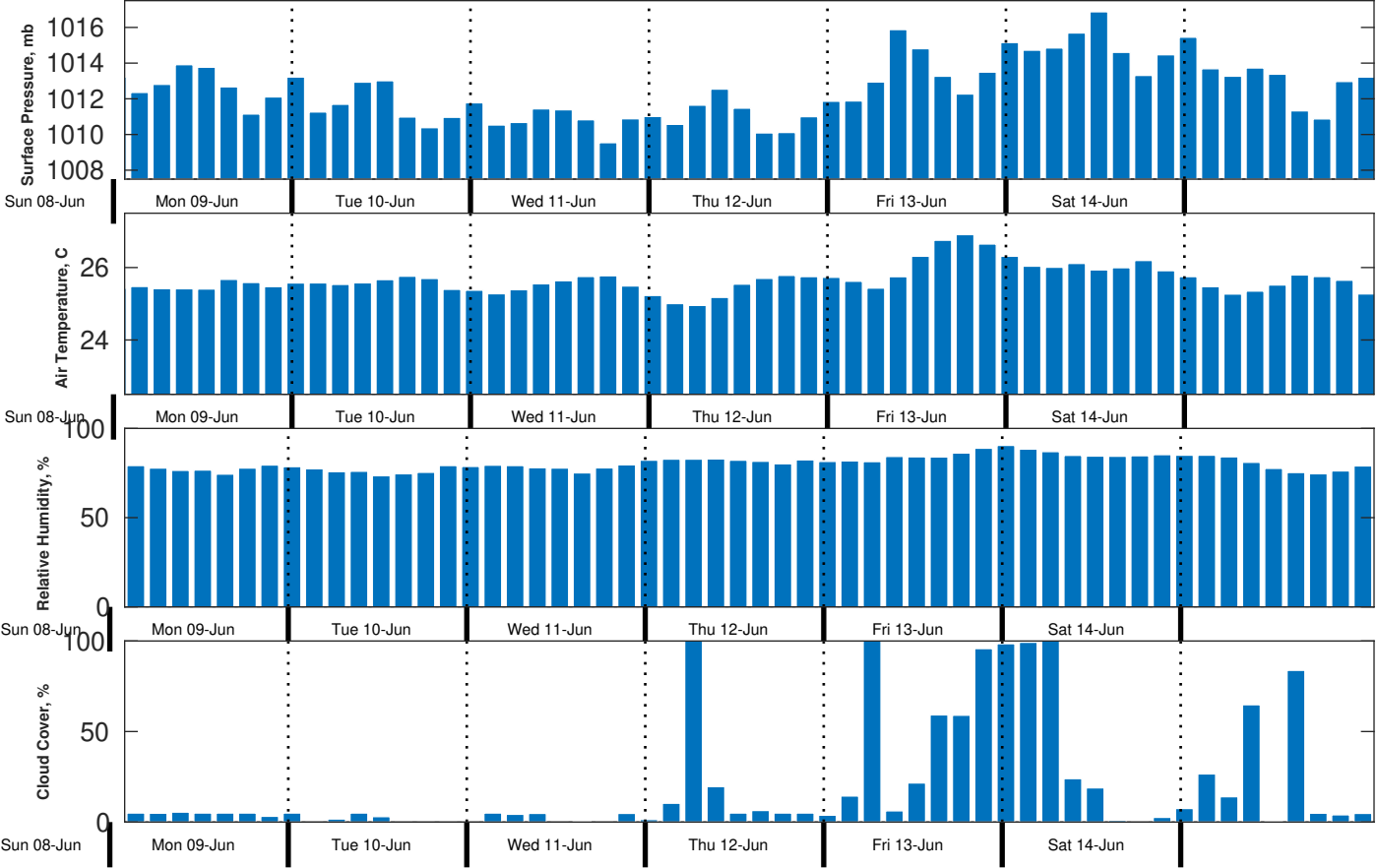
Met Forecast for Gyre from 08-Jun-2025 23:00:00 to 15-Jun-2025 23:00:00
