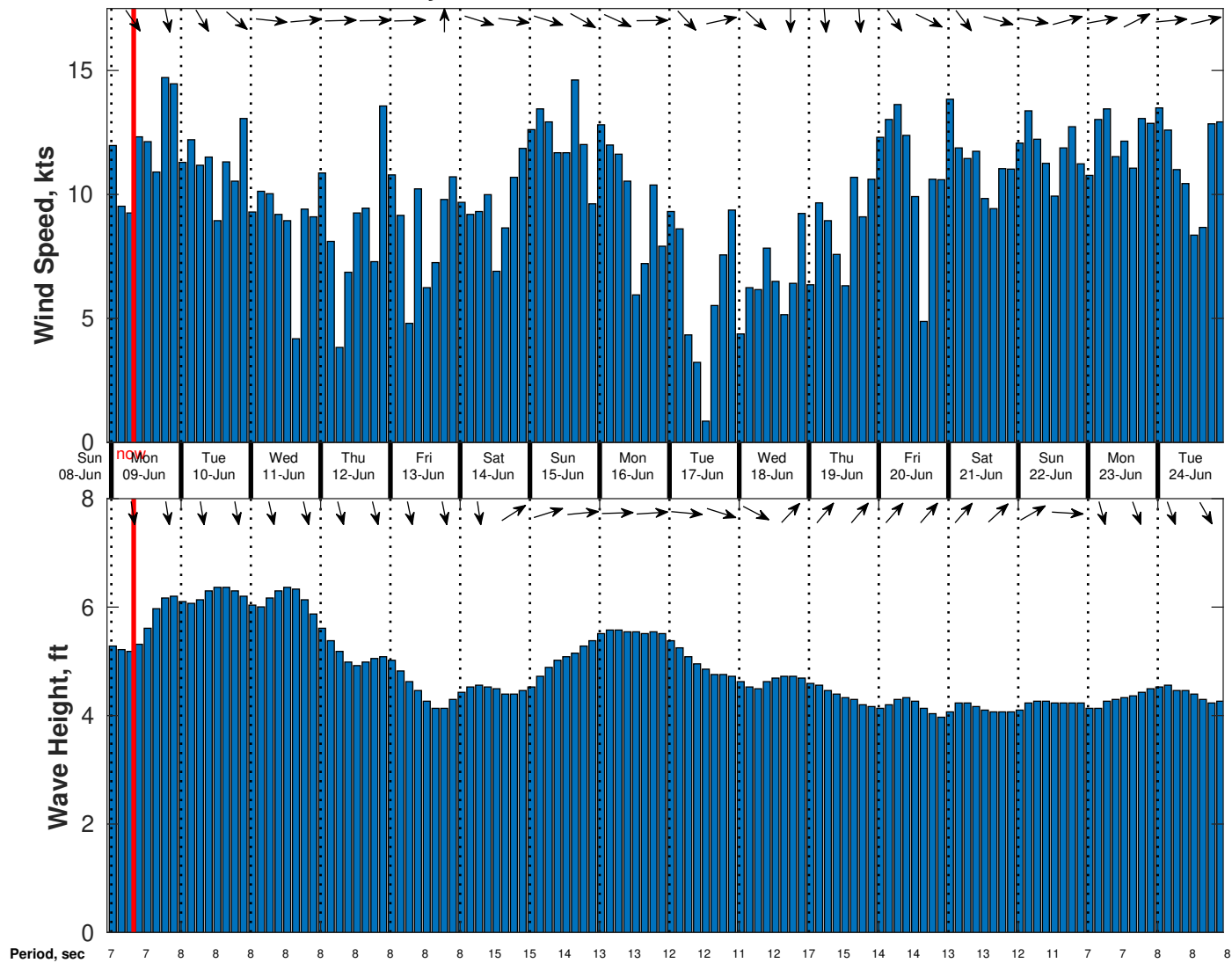
Wind & Wave Forecast for Gyre from 08-Jun-2025 23:00:00 to 24-Jun-2025 23:00:00
