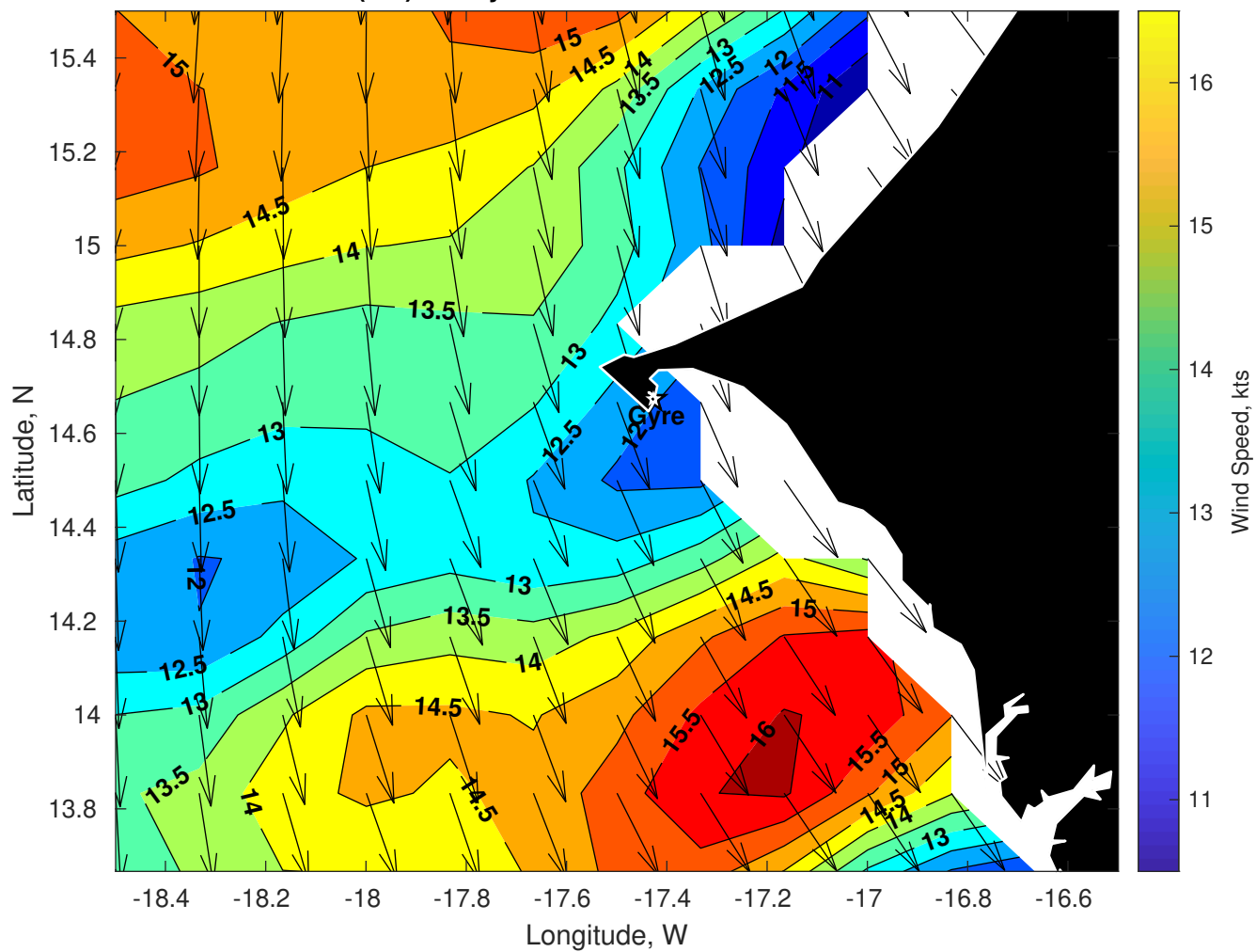
Winds (kts) for Gyre at 09-Jun-2025 09:00:00
