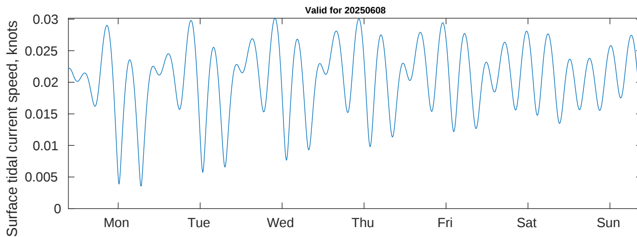
Tidal Currents and Heights for Benthic Solutions South Africa HF Site1 at 20250608
