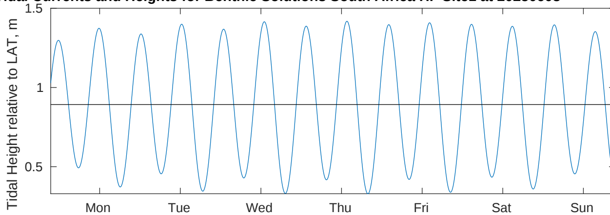
Tidal Currents and Heights for Benthic Solutions South Africa HF Site1 at 20250608
