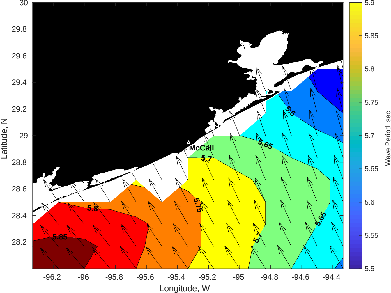
Wave Period (sec) for Brooks McCall at 10-Jun-2025 09:00:00
