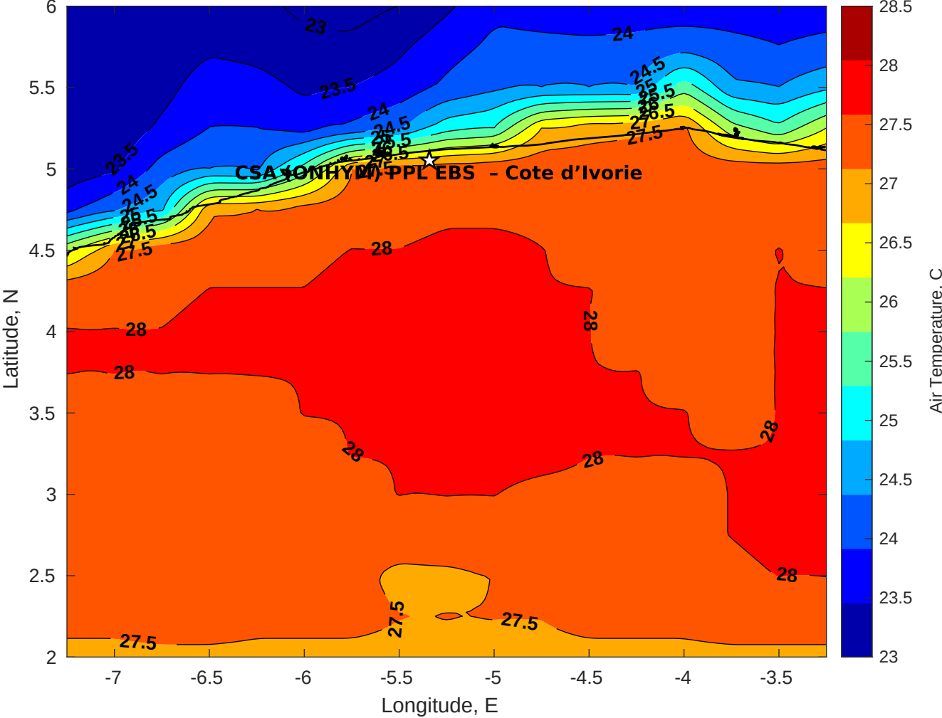
Air Temperature (C) for CSA (ONHYM) PPL EBS - Cote d'Ivoire at 08-Jun-2025
