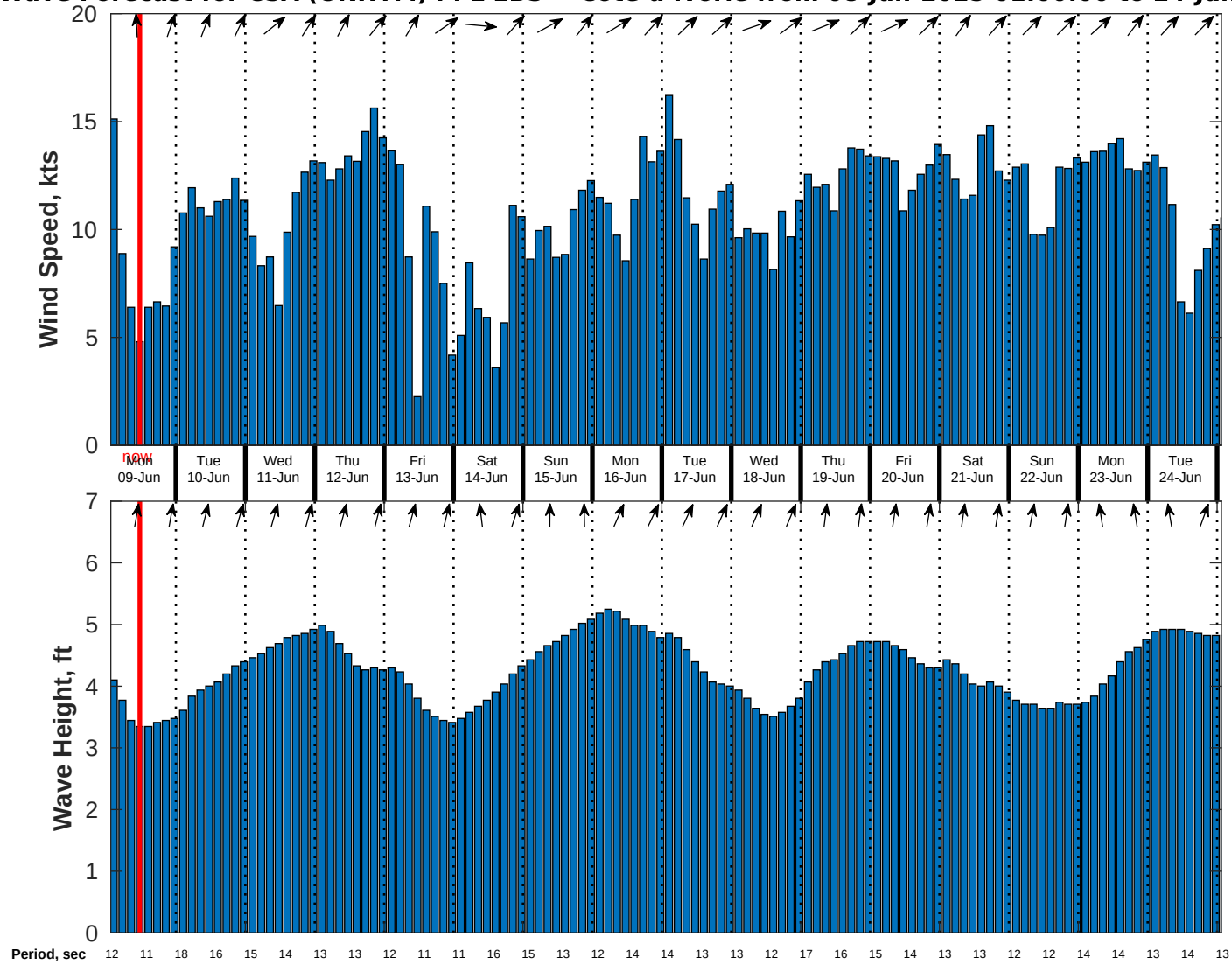
Wind & Wave Forecast for CSA (ONHYM) PPL EBS - Cote d'Ivoire from 08-Jun-2025 01:00:00 to 24-Jun-2025 01:00:00
