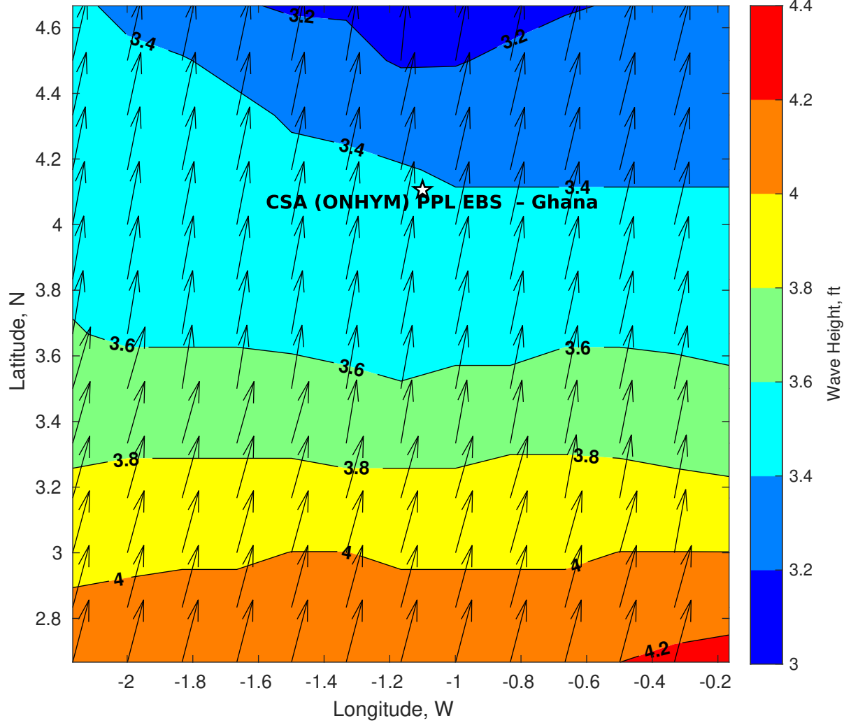
Wave Height (ft) for CSA (ONHYM) PPL EBS - Ghana at 08-Jun-2025 09:00:00
