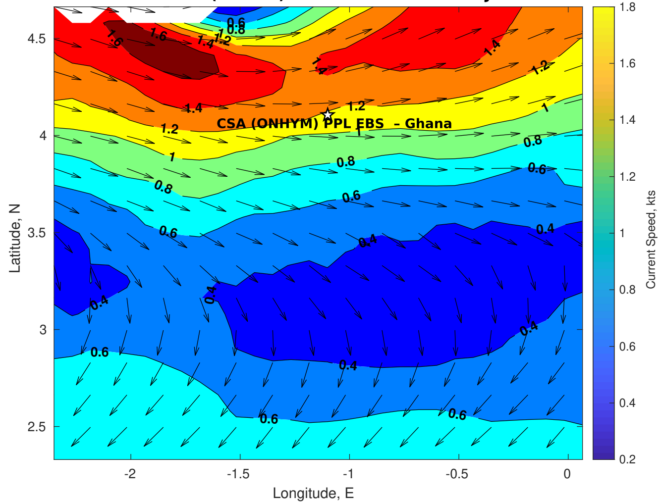
Surface Currents for CSA (ONHYM) PPL EBS - Ghana at 07-Jun-2025 00:00:00
