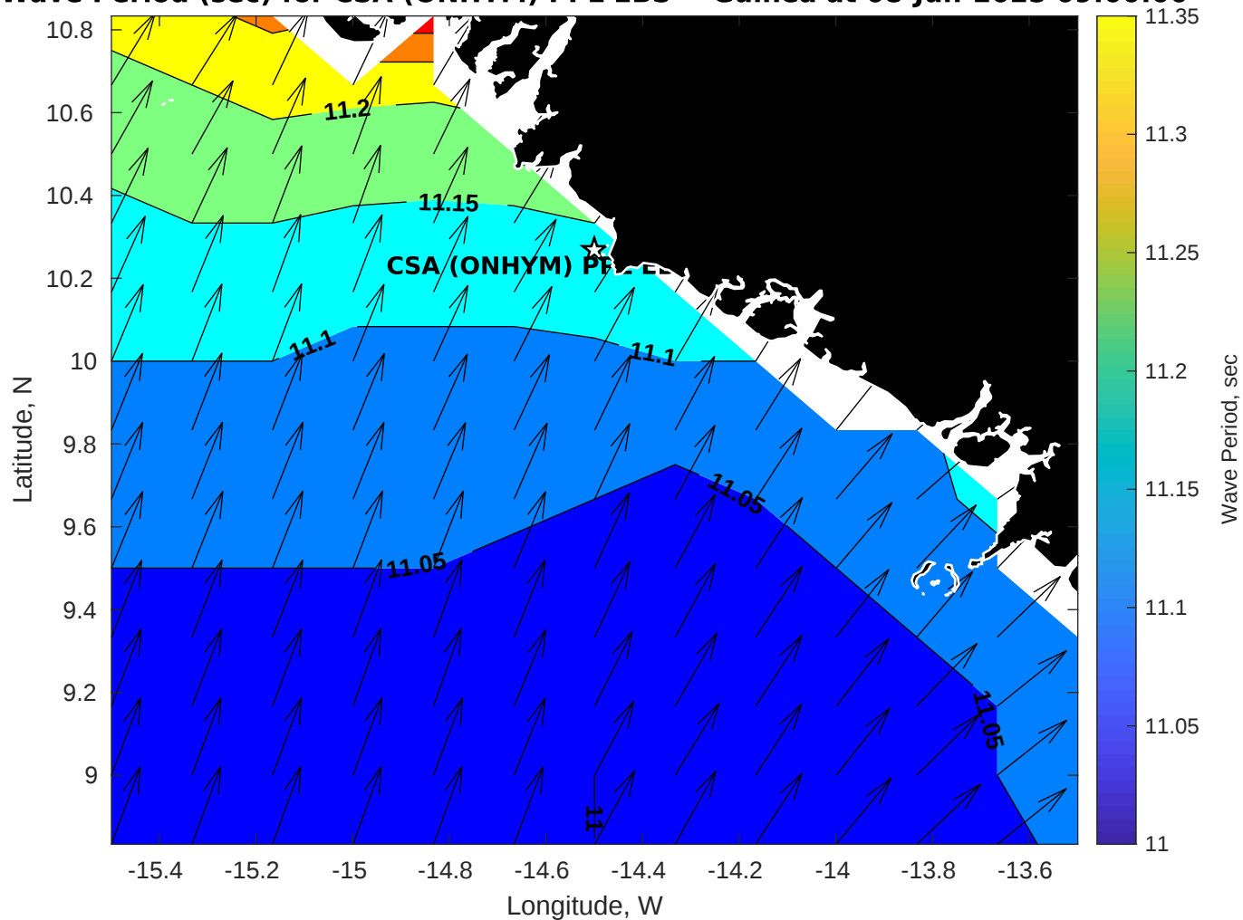
Wave Period (sec) for CSA (ONHYM) PPL EBS - Guinea at 08-Jun-2025 09:00:00
