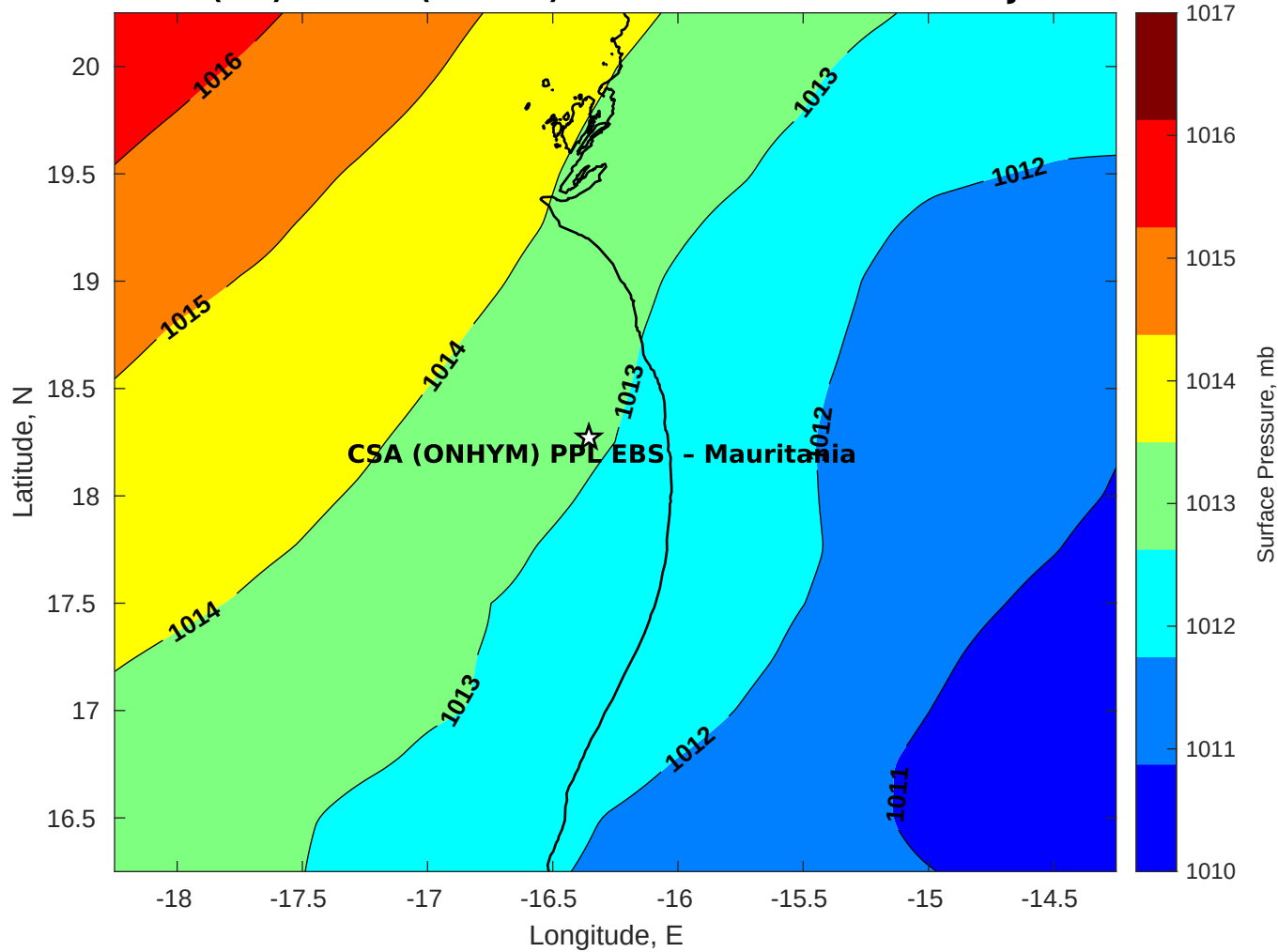
Surface Pressure (mb) for CSA (ONHYM) PPL EBS - Mauritania at 08-Jun-2025 00:00:00
