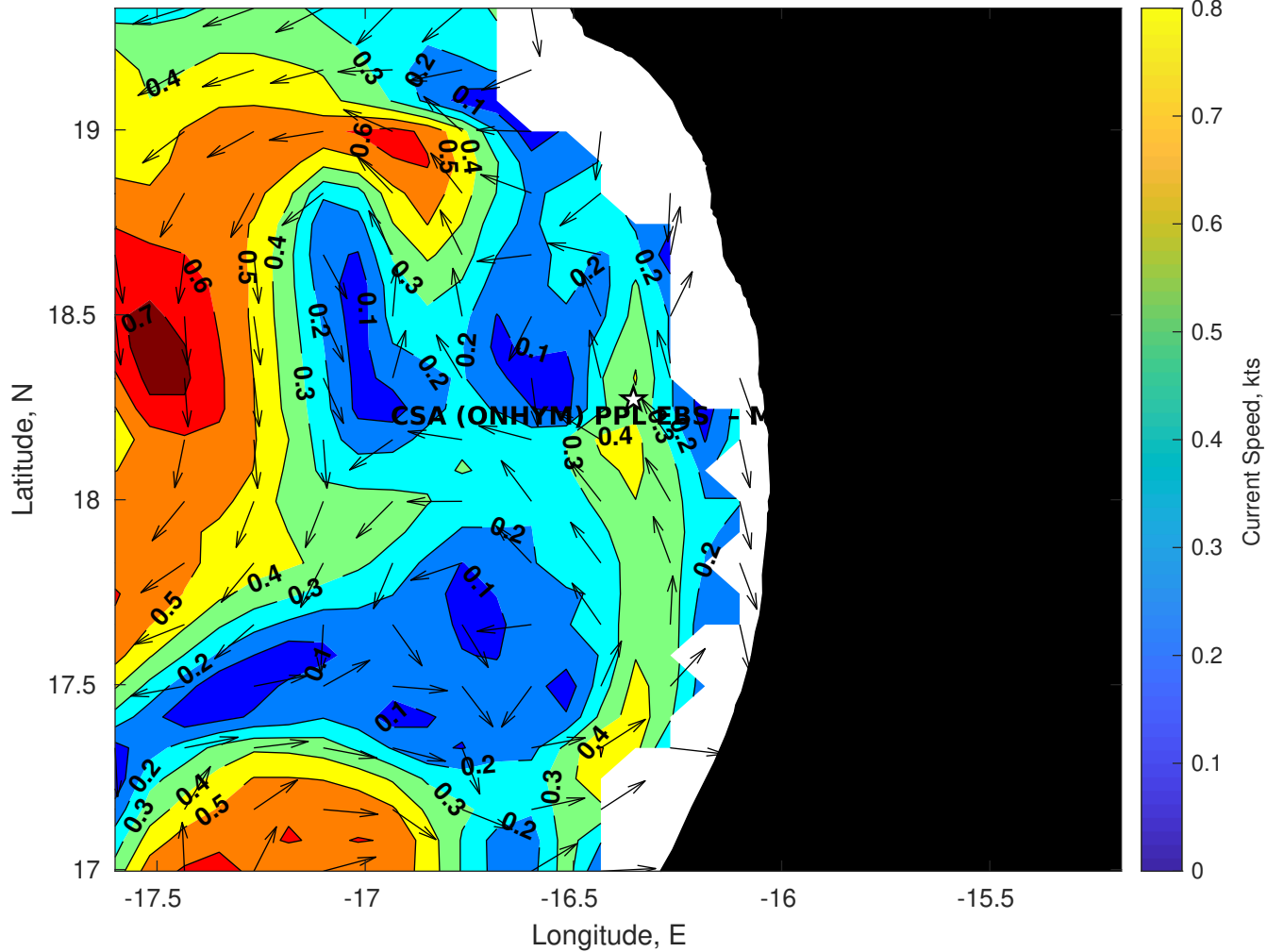
Surface Currents for CSA (ONHYM) PPL EBS - Mauritania at 07-Jun-2025 00:00:00
