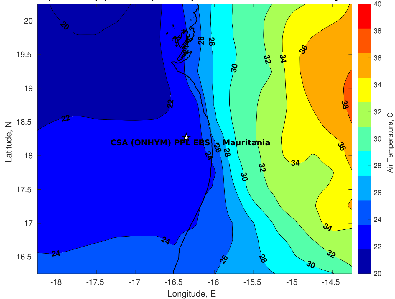
Air Temperature (C) for CSA (ONHYM) PPL EBS - Mauritania at 08-Jun-2025
