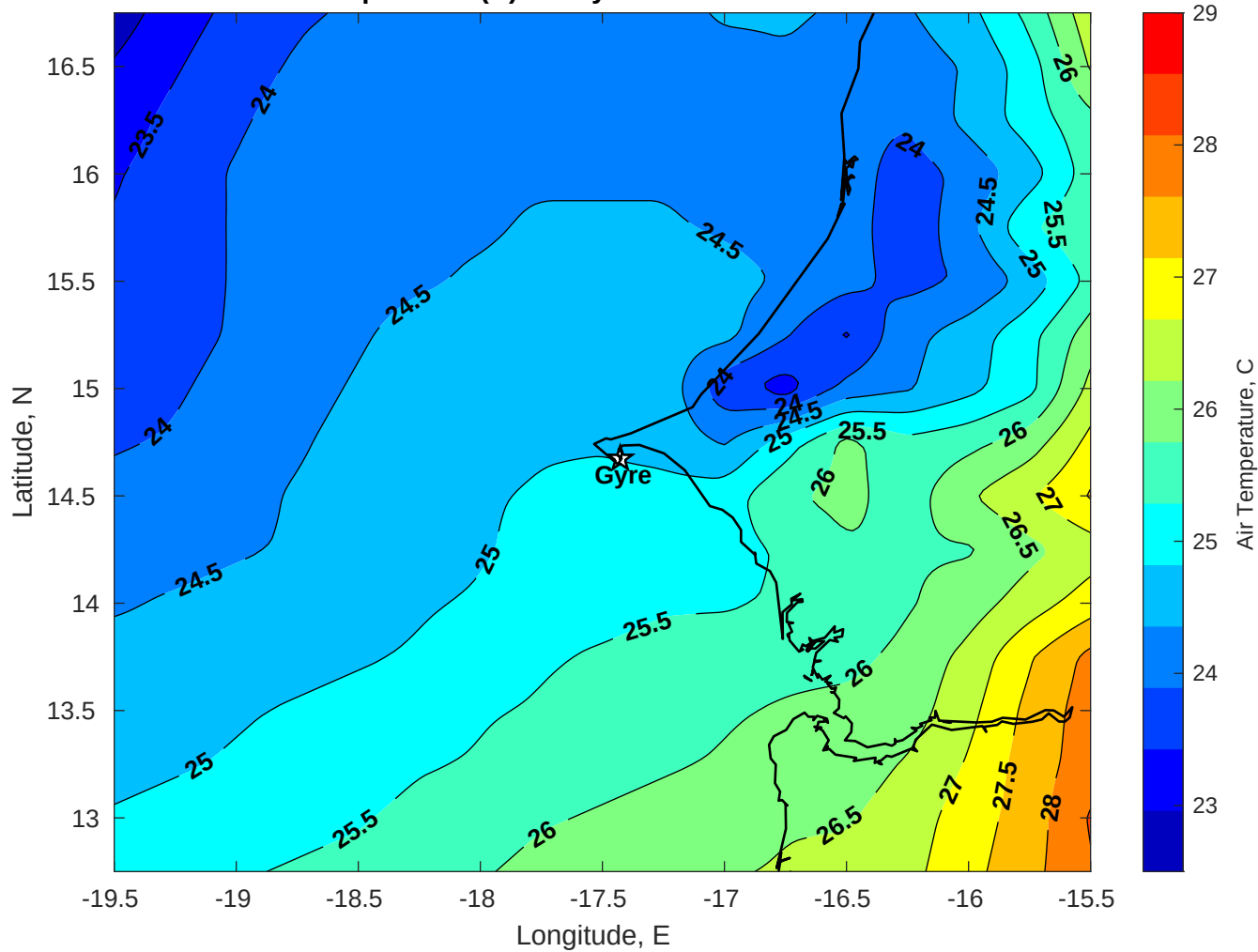
Air Temperature (C) for Gyre at 10-Jun-2025
