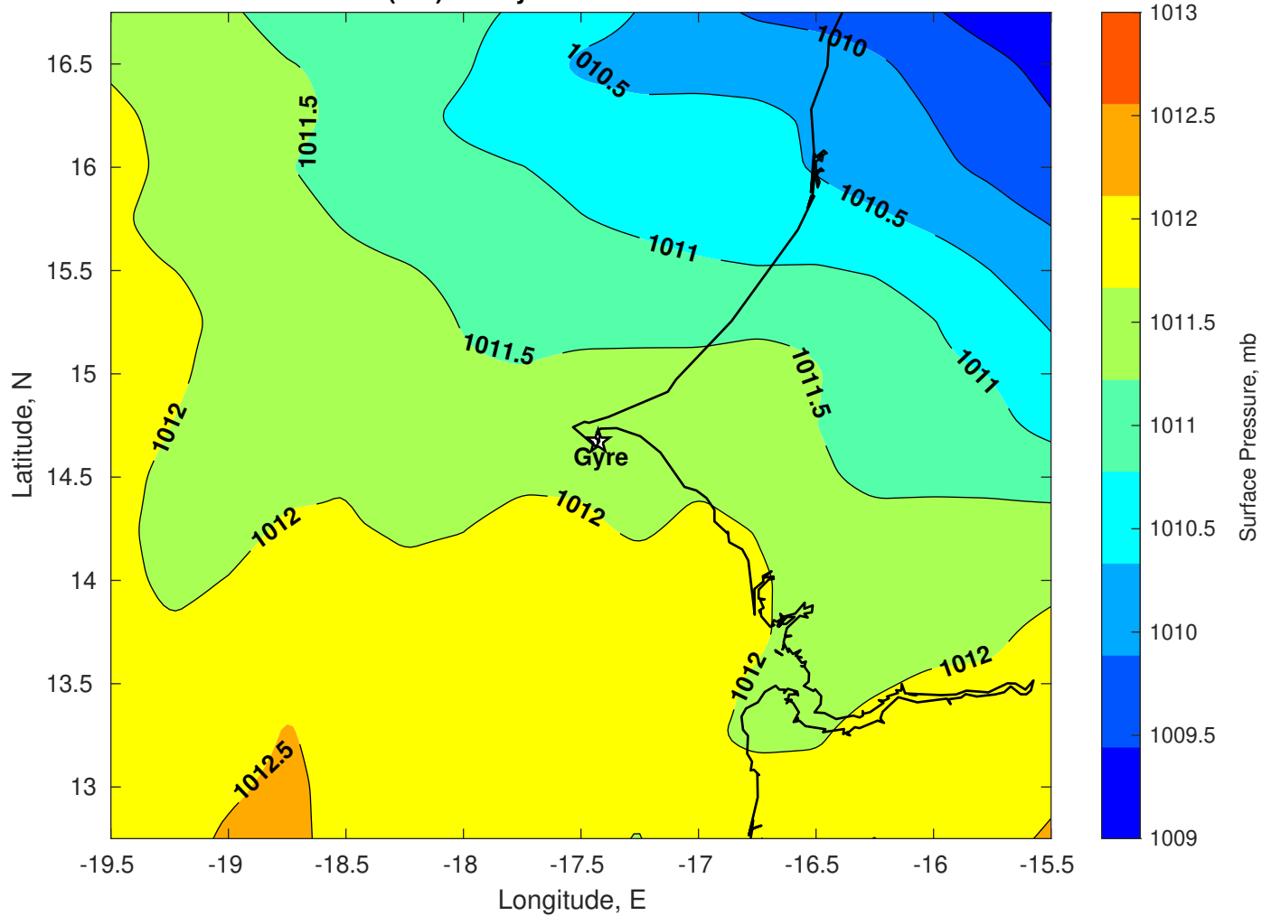
Surface Pressure (mb) for Gyre at 12-Jun-2025 00:00:00
