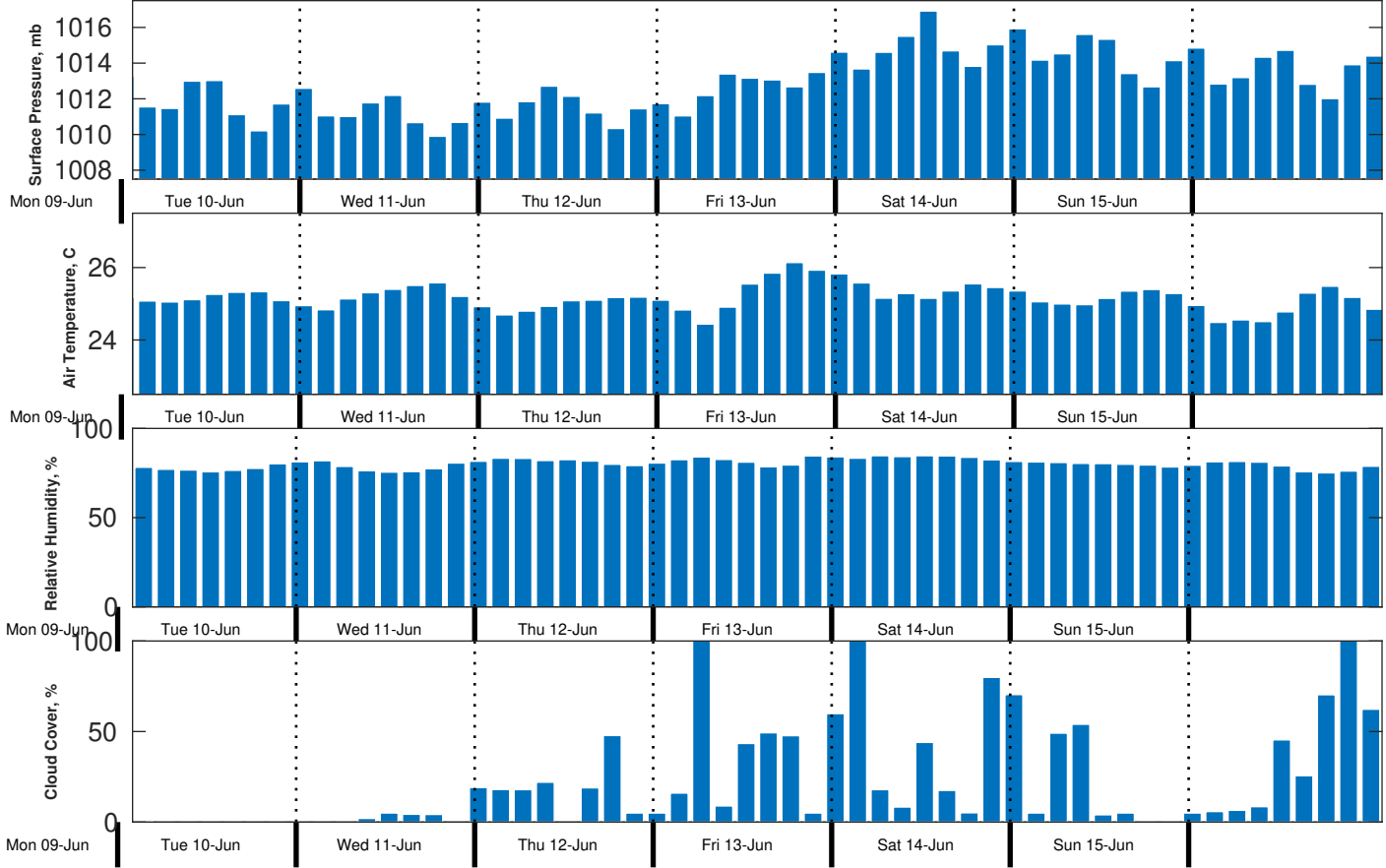
Met Forecast for Gyre from 09-Jun-2025 23:00:00 to 16-Jun-2025 23:00:00
