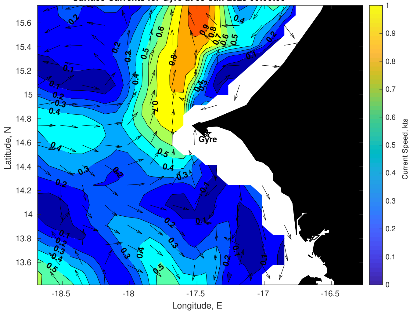
Surface Currents for Gyre at 09-Jun-2025 00:00:00
