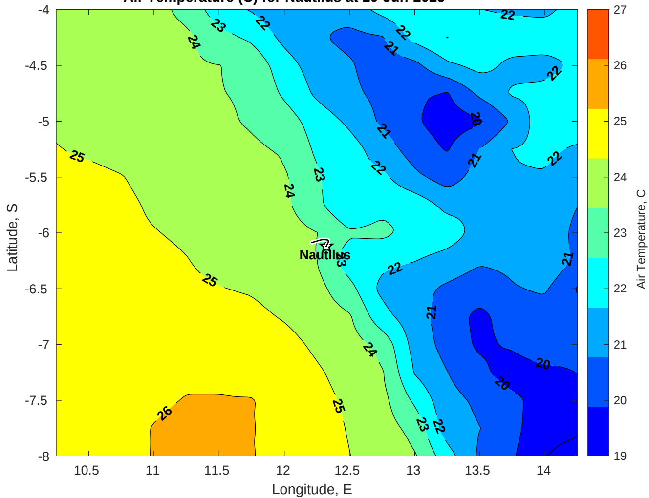
Air Temperature (C) for Nautilus at 10-Jun-2025
