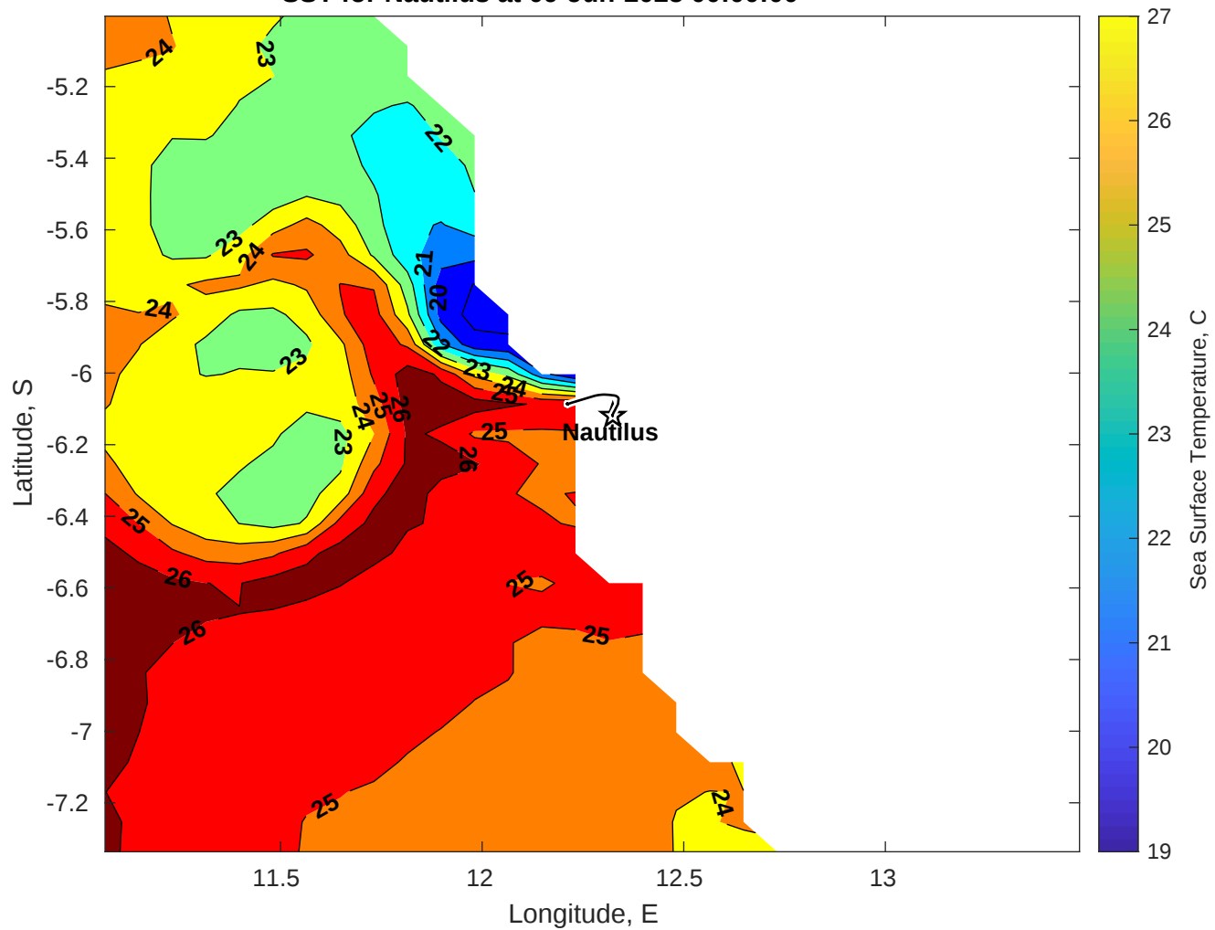
SST for Nautilus at 09-Jun-2025 00:00:00
