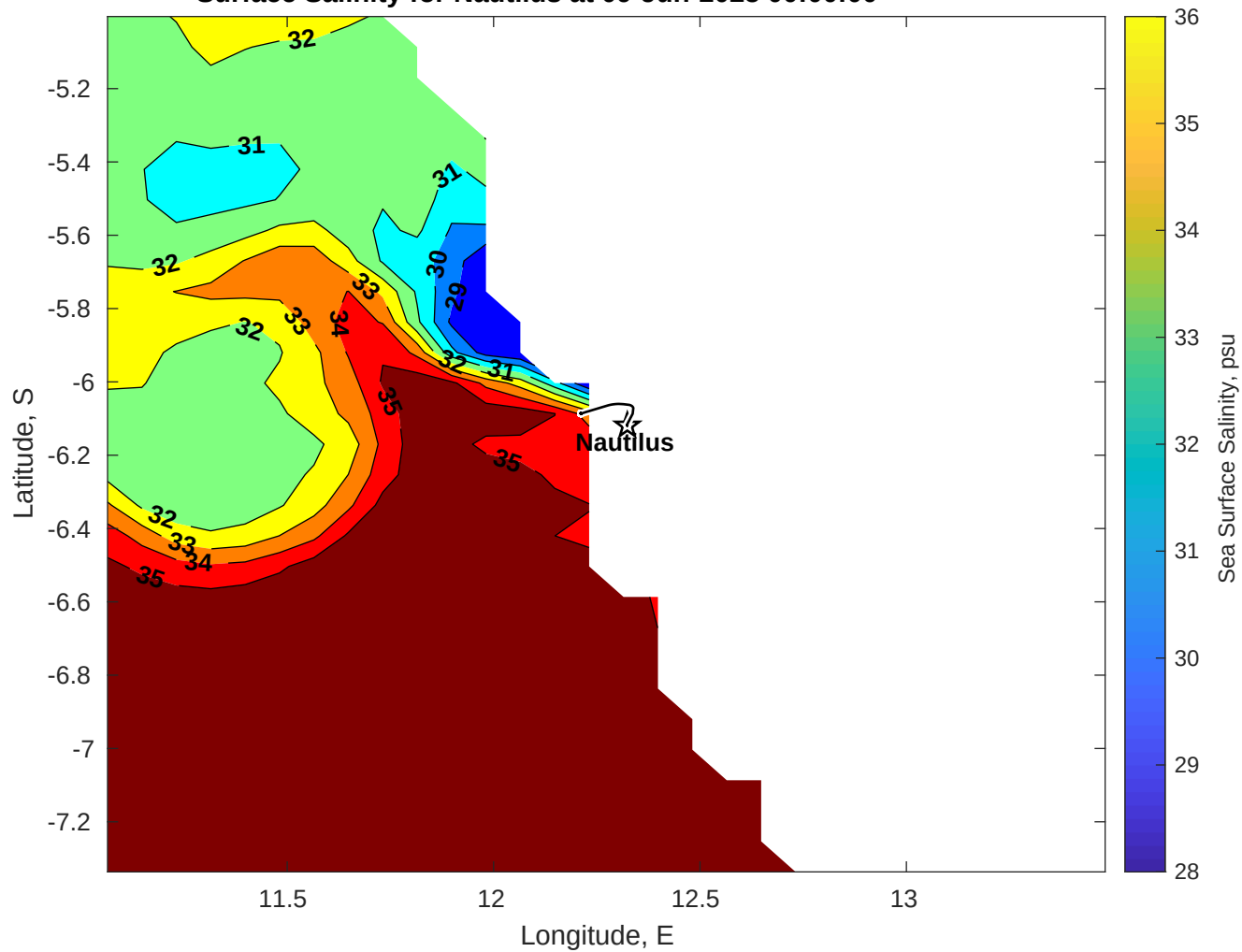
Surface Salinity for Nautilus at 09-Jun-2025 00:00:00
