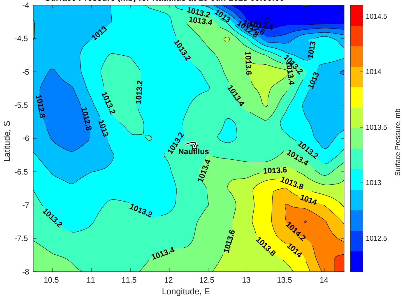
Surface Pressure (mb) for Nautilus at 10-Jun-2025 00:00:00
