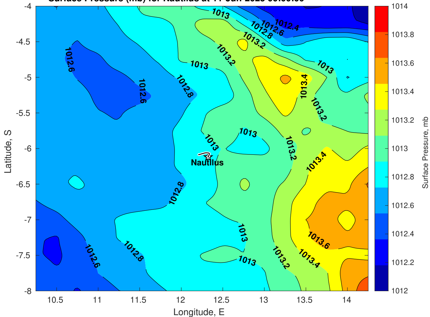
Surface Pressure (mb) for Nautilus at 11-Jun-2025 00:00:00
