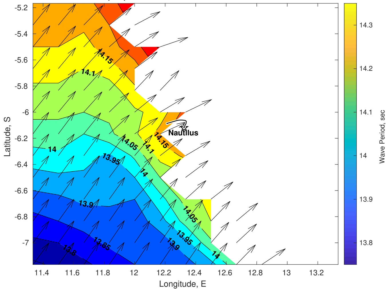
Wave Period (sec) for Nautilus at 10-Jun-2025 09:00:00
