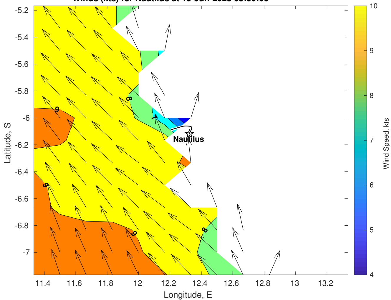
Winds (kts) for Nautilus at 10-Jun-2025 09:00:00
