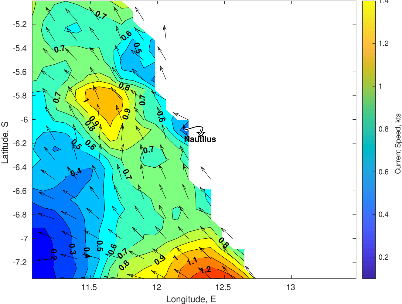
Surface Currents for Nautilus at 09-Jun-2025 00:00:00
