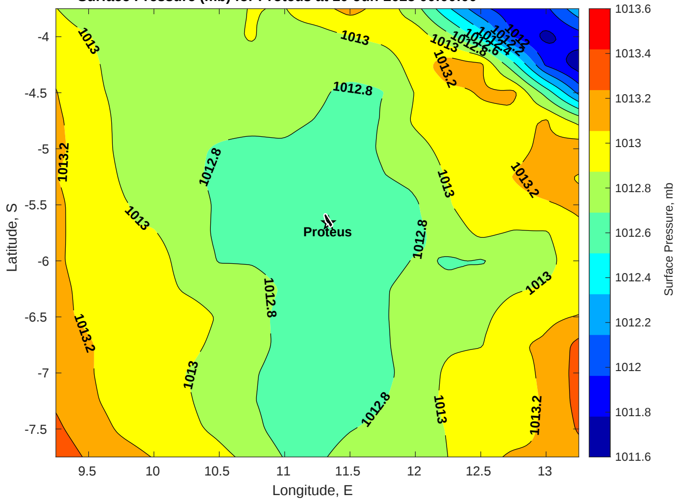
Surface Pressure (mb) for Proteus at 10-Jun-2025 00:00:00
