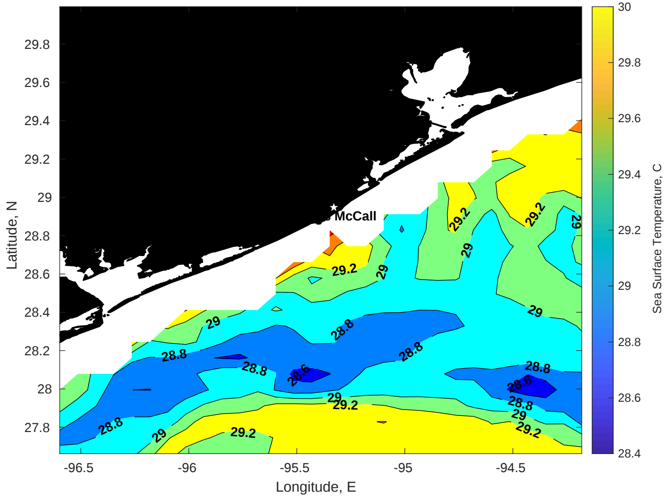
SST for Brooks McCall at 10-Jun-2025 00:00:00
