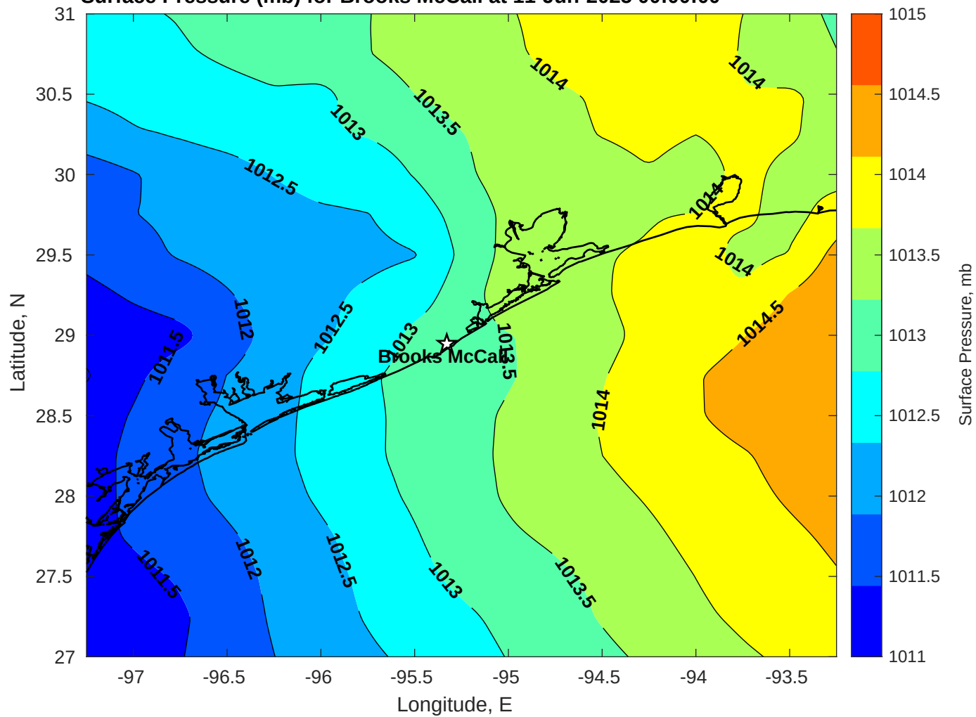
Surface Pressure (mb) for Brooks McCall at 11-Jun-2025 00:00:00
