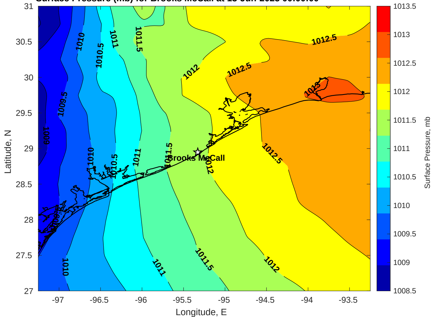
Surface Pressure (mb) for Brooks McCall at 13-Jun-2025 00:00:00
