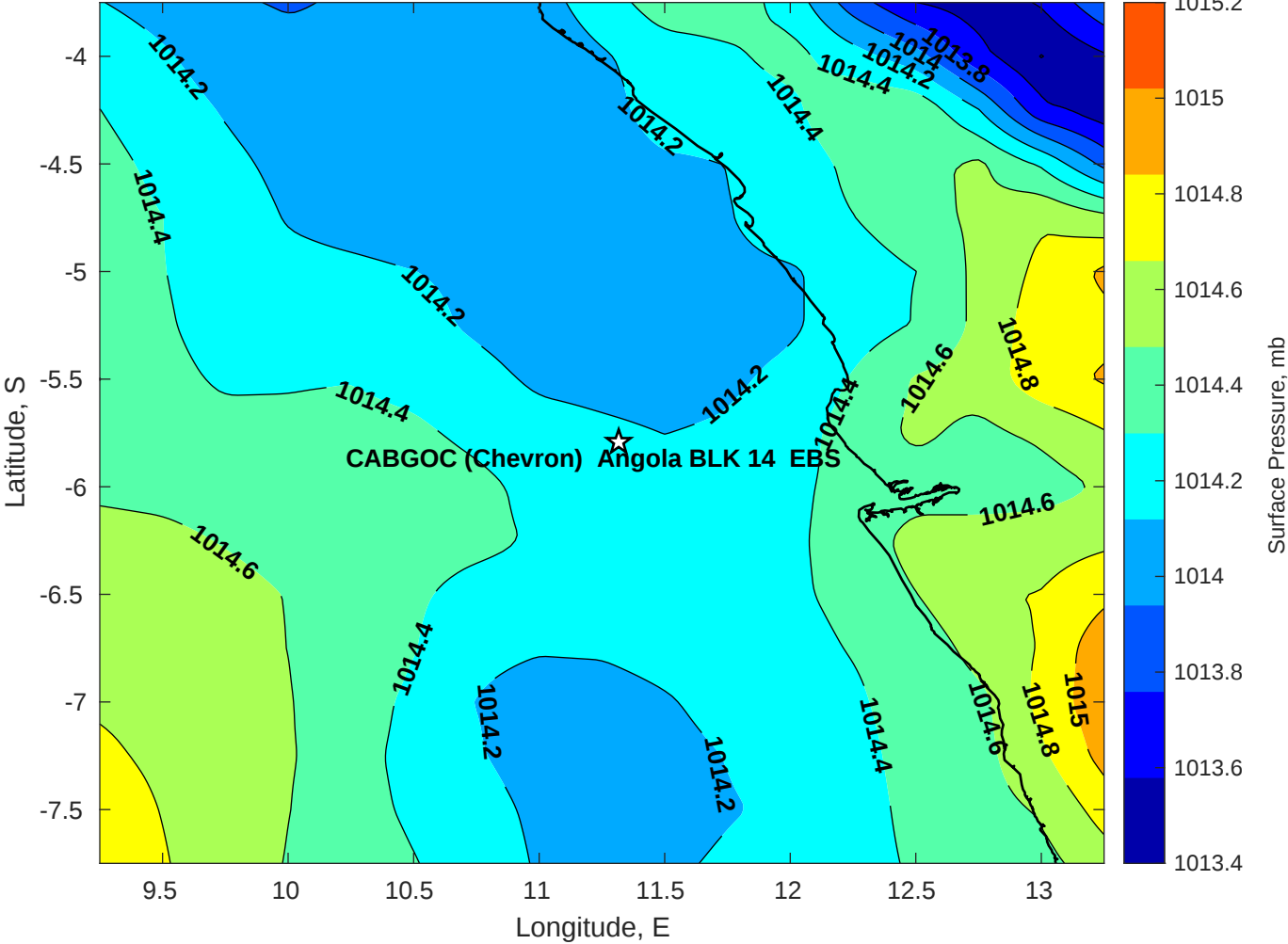
Surface Pressure (mb) for CABGOC (Chevron) Angola BLK 14 EBS at 08-Jun-2025 00:00:00
