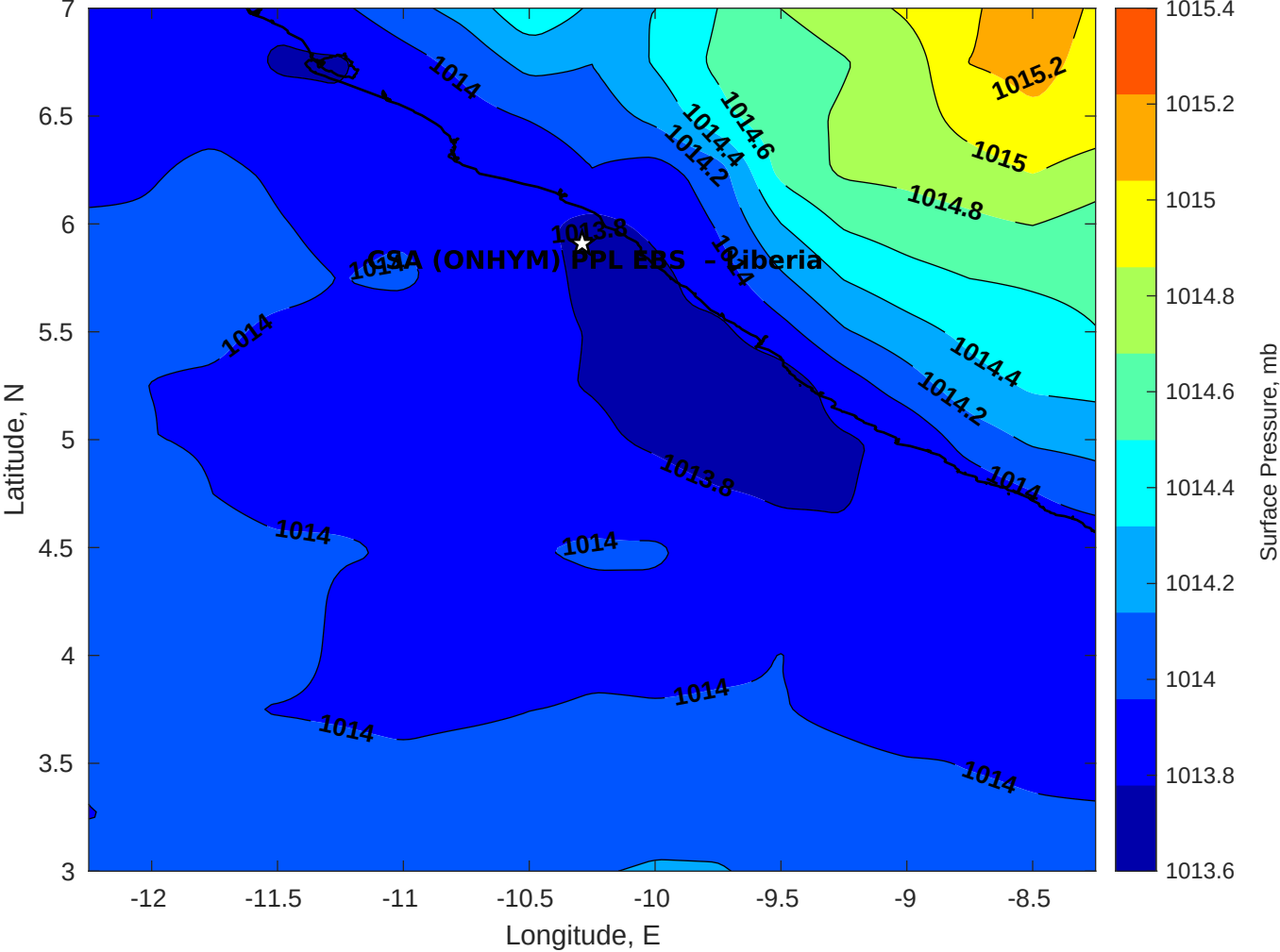
Surface Pressure (mb) for CSA (ONHYM) PPL EBS - Liberia at 08-Jun-2025 00:00:00
