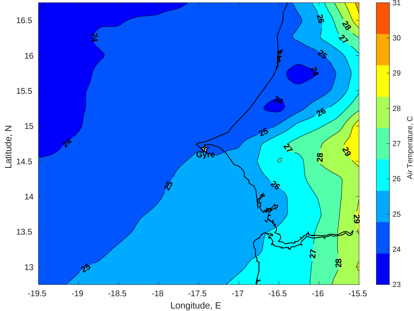
Air Temperature (C) for Gyre at 11-Jun-2025
