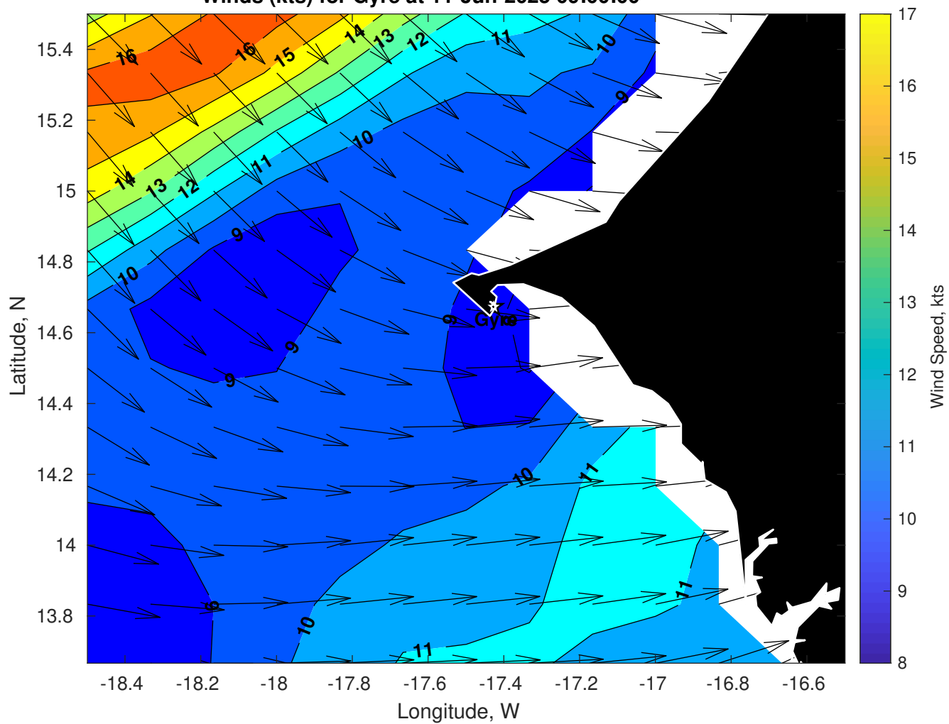
Winds (kts) for Gyre at 11-Jun-2025 09:00:00
