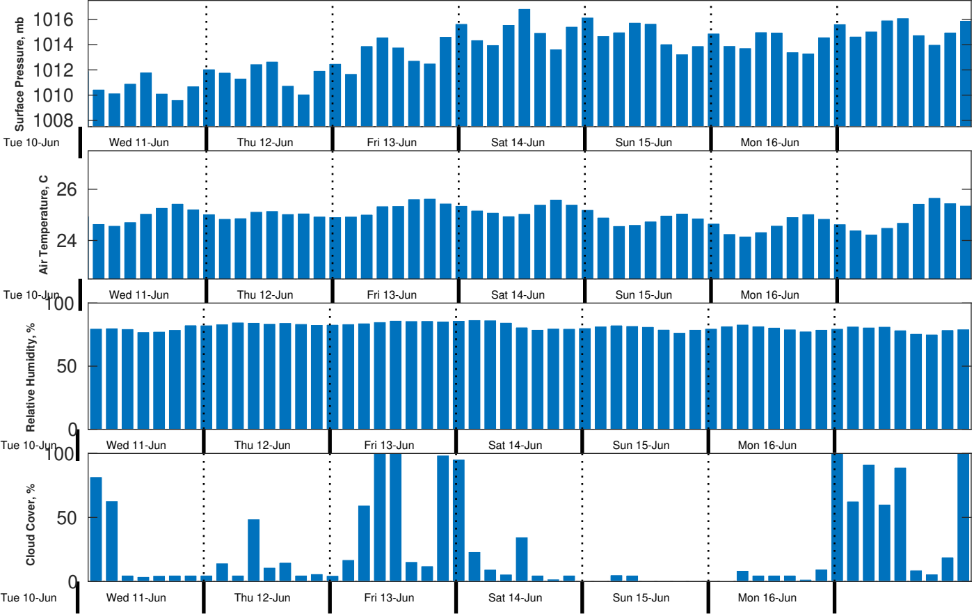
Met Forecast for Gyre from 10-Jun-2025 23:00:00 to 17-Jun-2025 23:00:00
