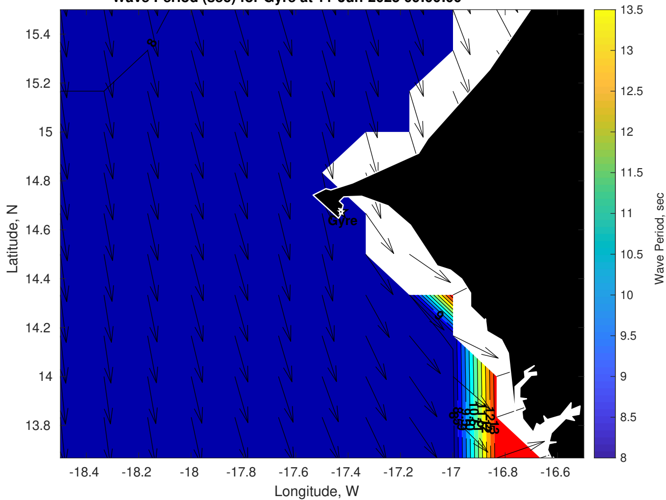
Wave Period (sec) for Gyre at 11-Jun-2025 09:00:00
