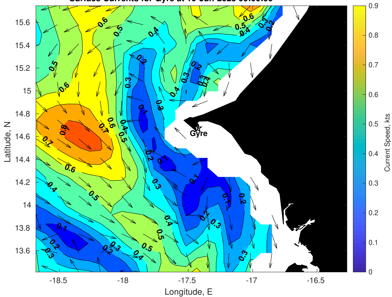
Surface Currents for Gyre at 10-Jun-2025 00:00:00
