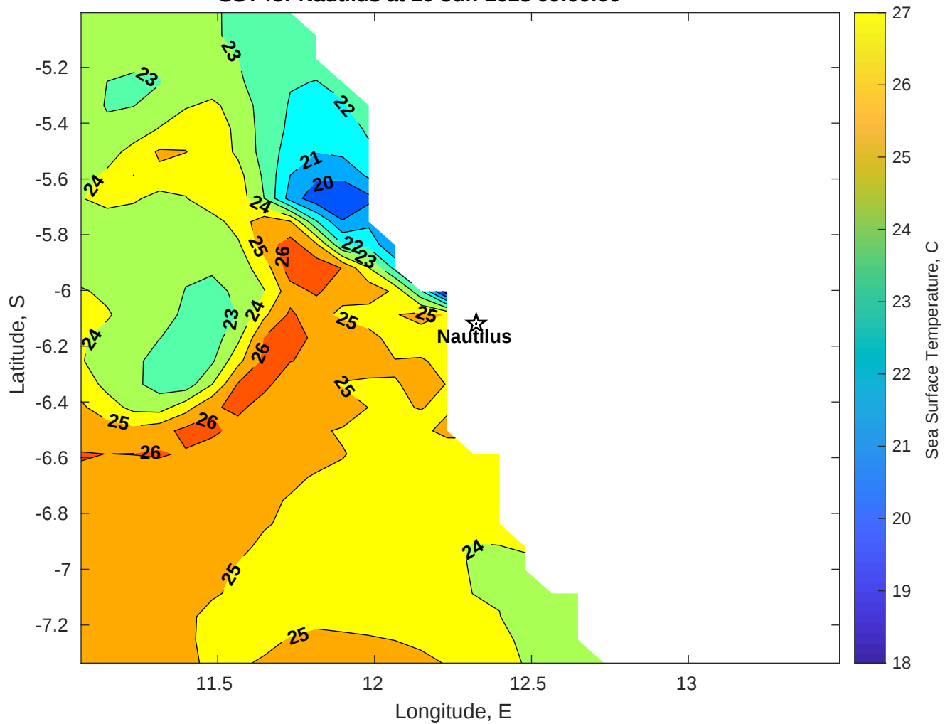
SST for Nautilus at 10-Jun-2025 00:00:00
