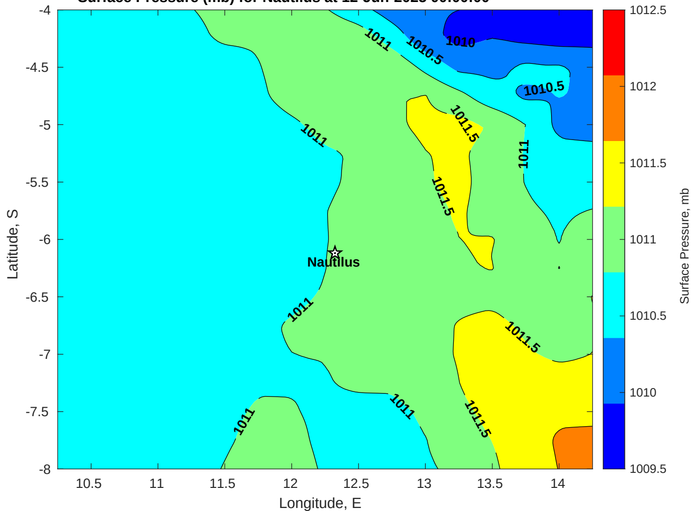
Surface Pressure (mb) for Nautilus at 12-Jun-2025 00:00:00
