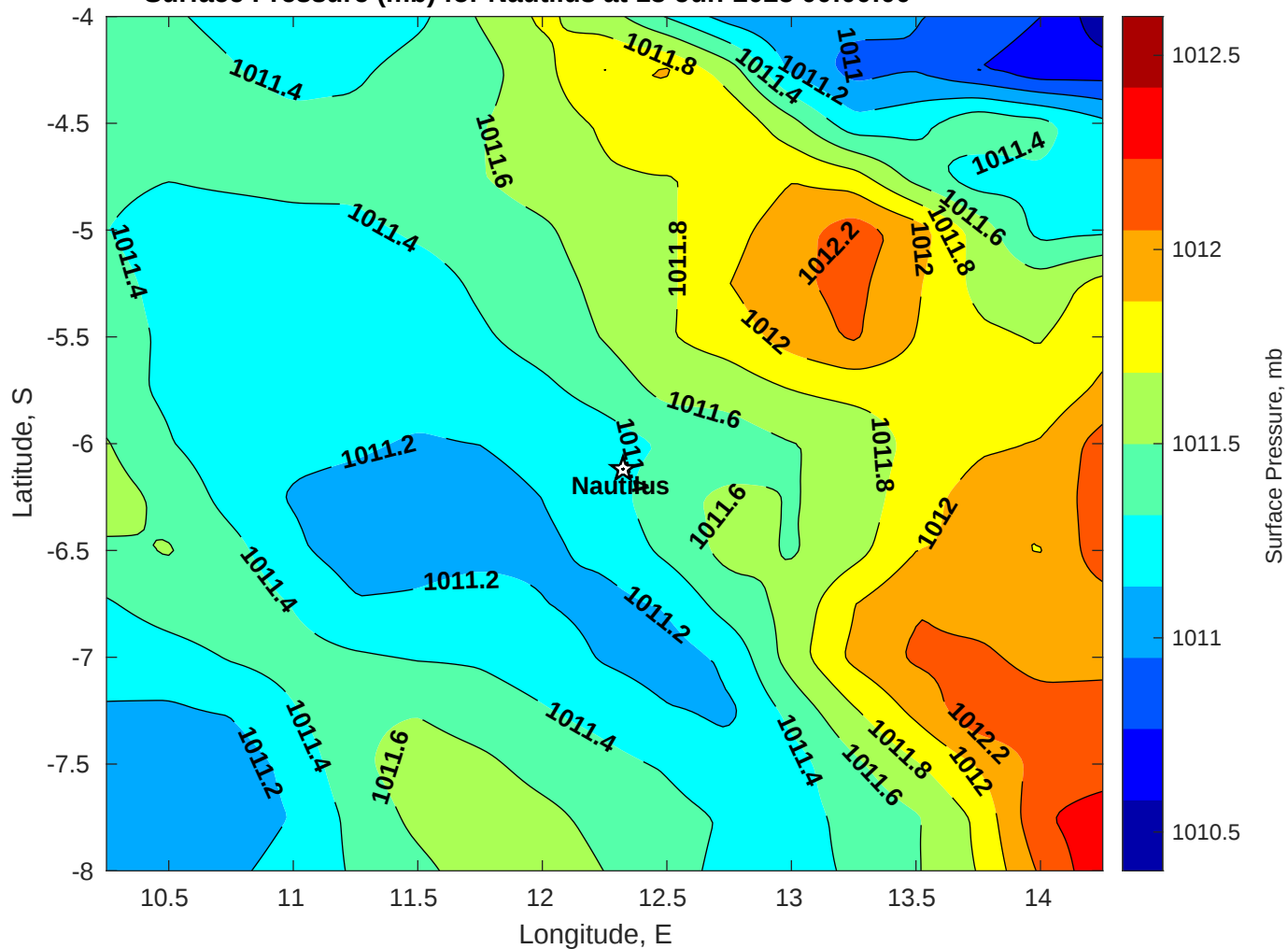
Surface Pressure (mb) for Nautilus at 13-Jun-2025 00:00:00
