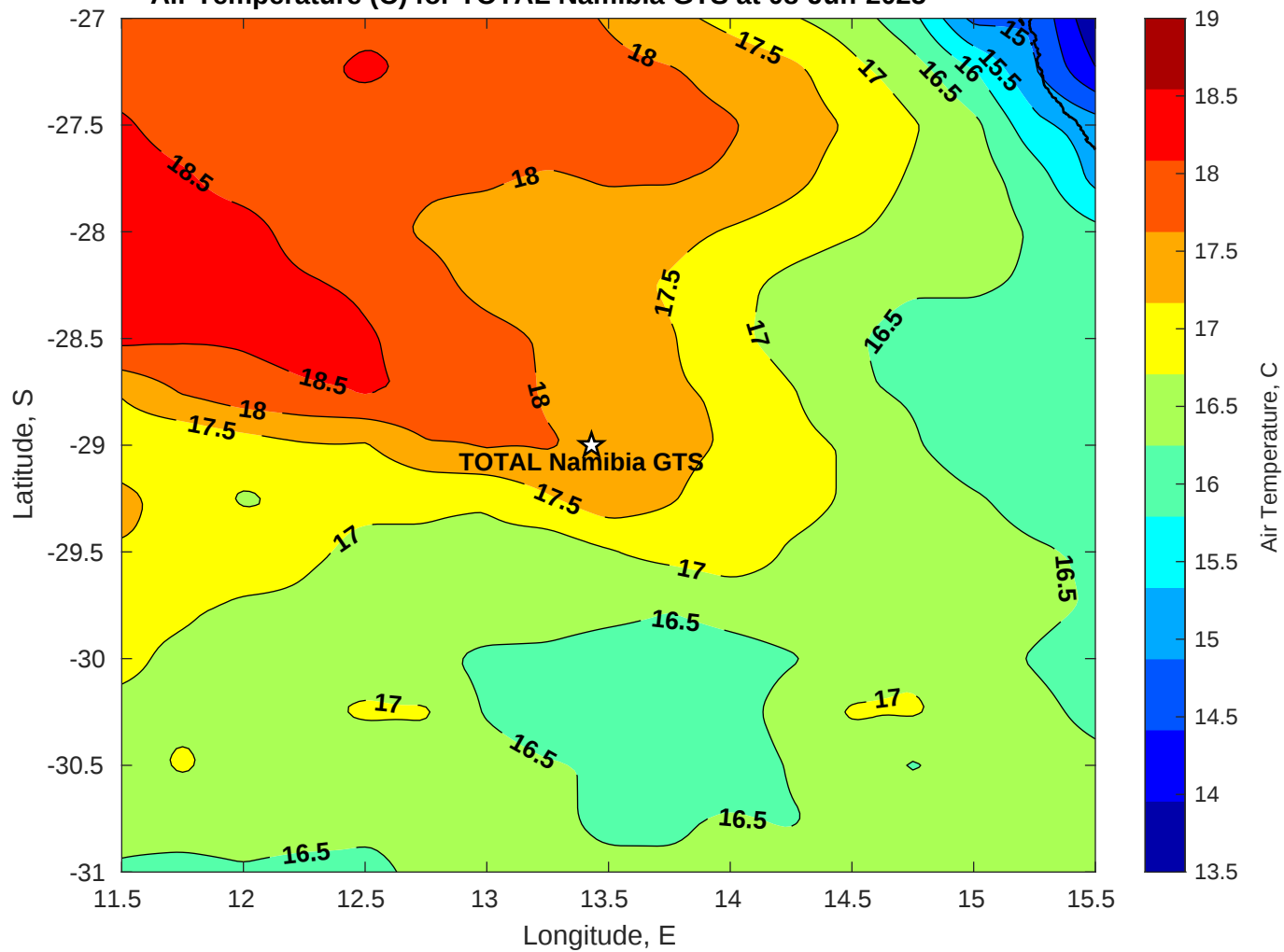
Air Temperature (C) for TOTAL Namibia GTS at 08-Jun-2025
