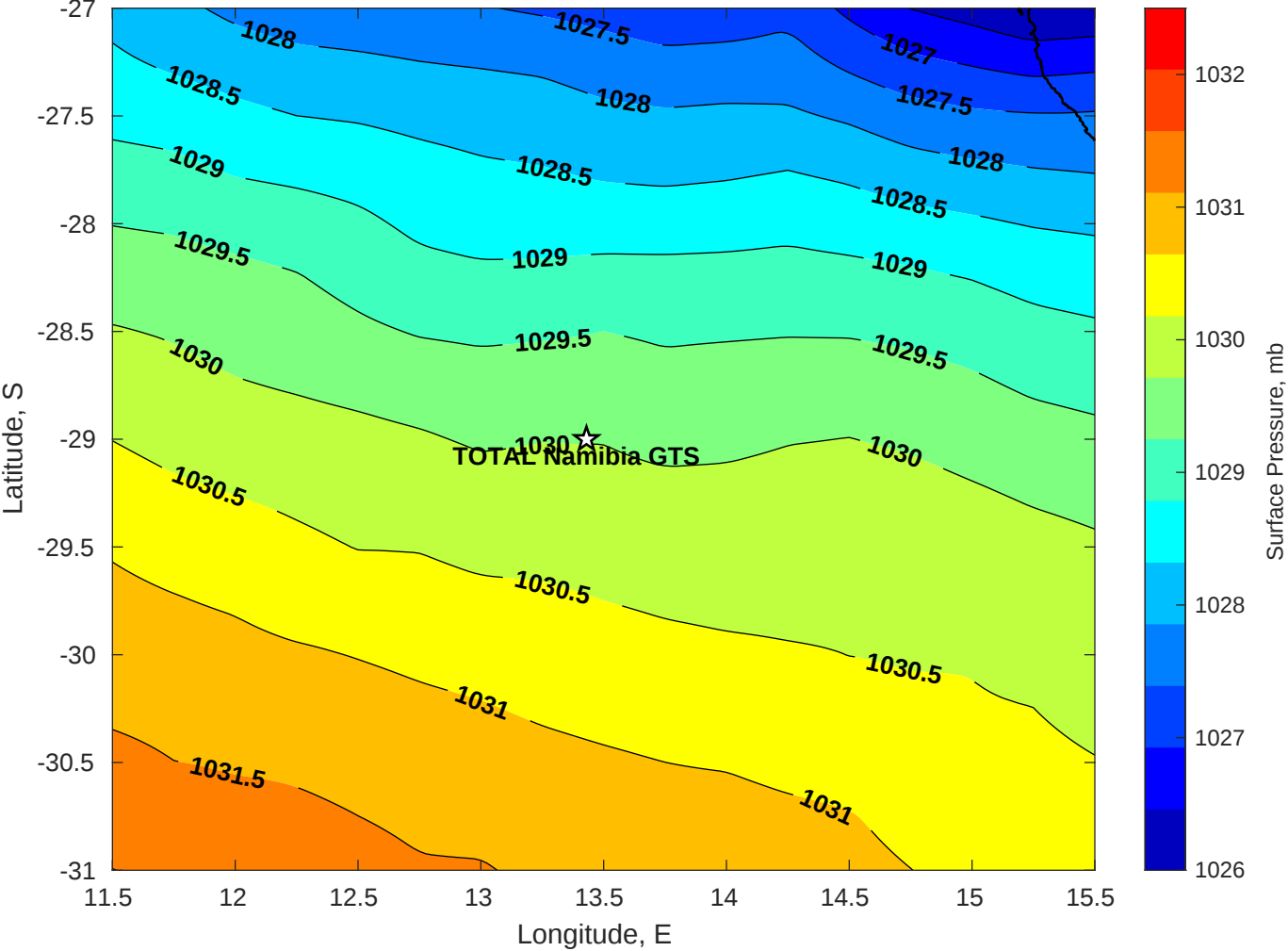
Surface Pressure (mb) for TOTAL Namibia GTS at 10-Jun-2025 00:00:00
