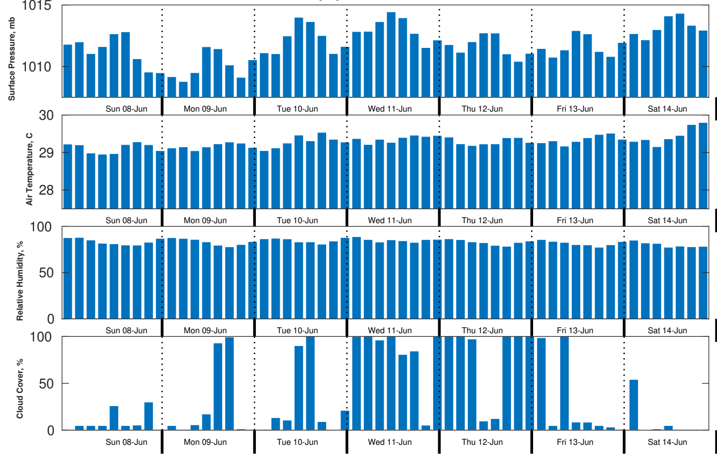
Met Forecast for Tampnet P2378 South Texas Cable Route Geophysical from 08-Jun-2025 00:00:00 to 15-Jun-2025 00:00:00
