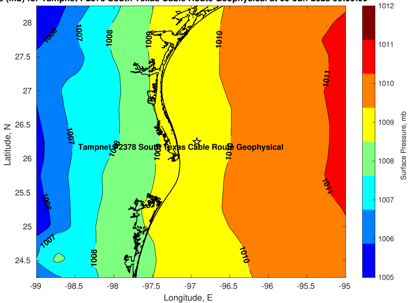
Pressure (mb) for Tampnet P2378 South Texas Cable Route Geophysical at 09-Jun-2025 00:00:00
