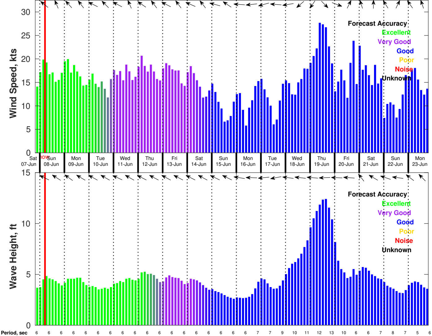
Wind & Wave Forecast for Tampnet P2378 South Texas Cable Route Geophysical from 07-Jun-2025 20:00:00 to 23-Jun-2025 20:00:00
