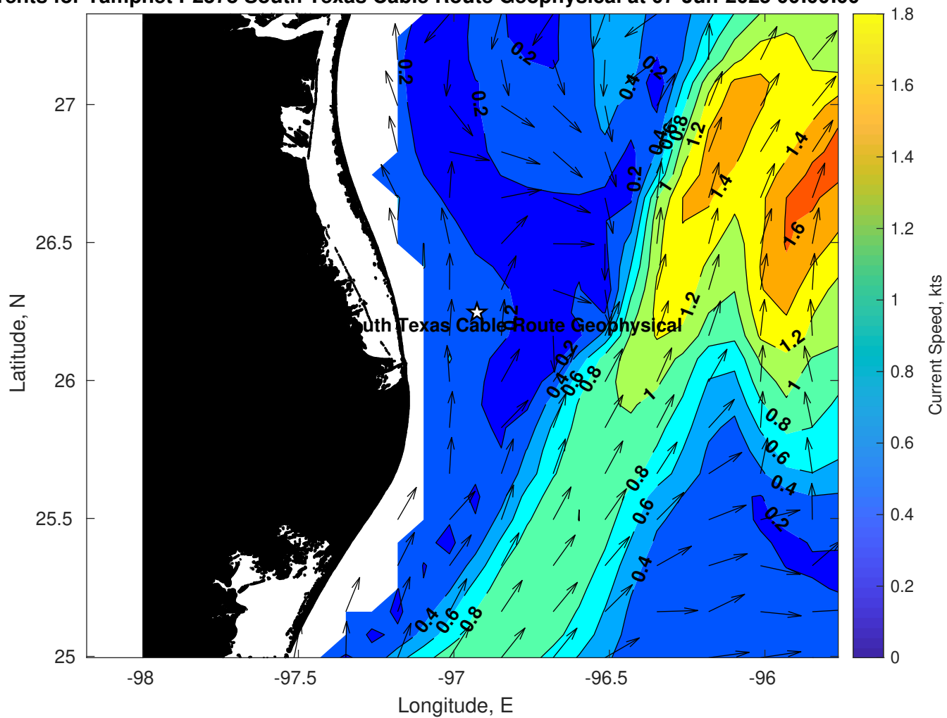
Surface Currents for Tampnet P2378 South Texas Cable Route Geophysical at 07-Jun-2025 00:00:00
