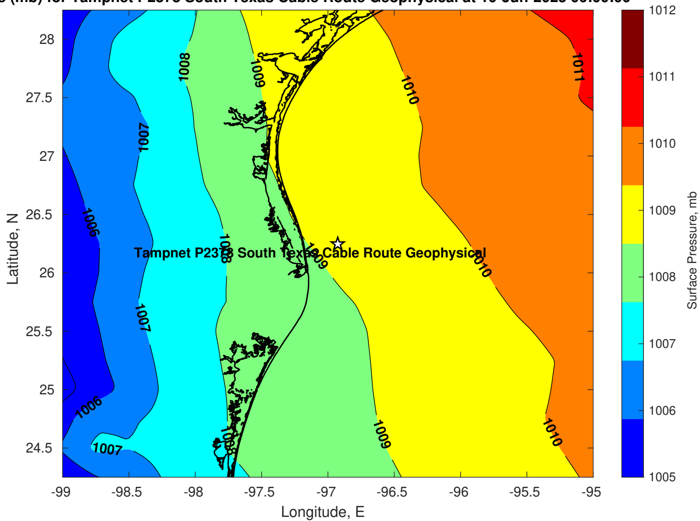
Pressure (mb) for Tampnet P2378 South Texas Cable Route Geophysical at 10-Jun-2025 00:00:00
