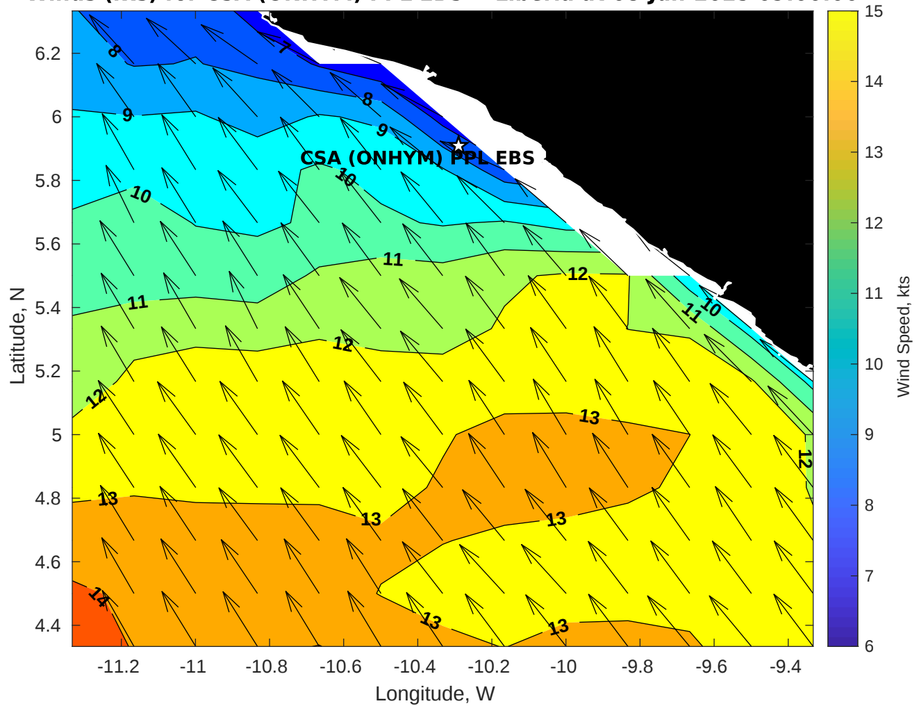
Winds (kts) for CSA (ONHYM) PPL EBS - Liberia at 08-Jun-2025 09:00:00
