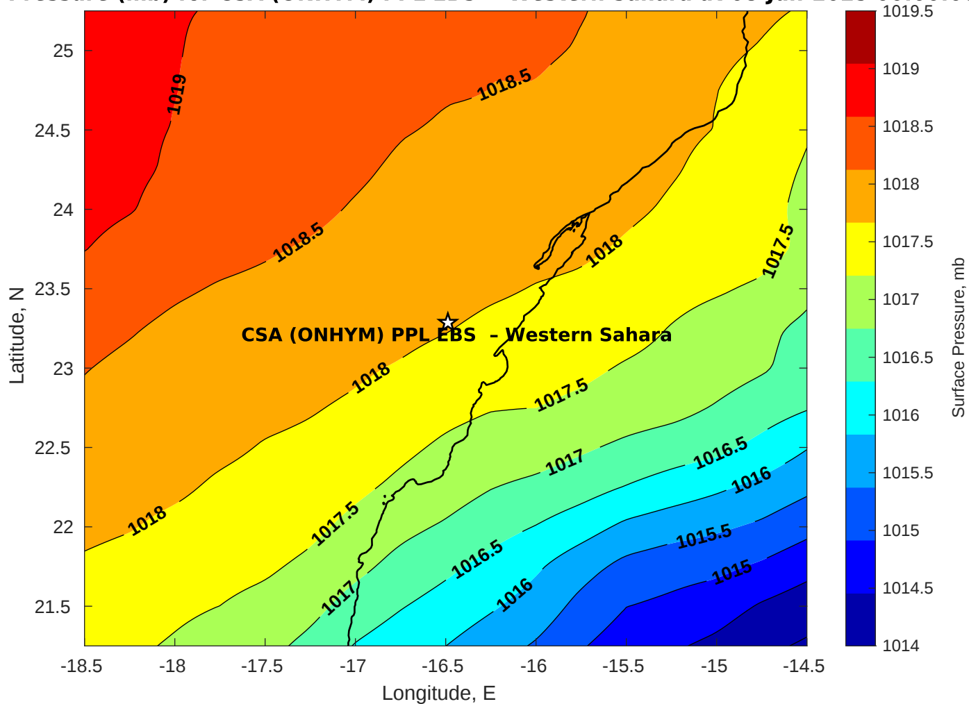
Surface Pressure (mb) for CSA (ONHYM) PPL EBS - Western Sahara at 08-Jun-2025 00:00:00
